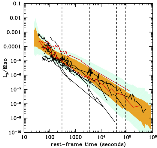
Figure 1: Best fit of the X-ray luminosity light curves of the SGRBs with redshift of the S-BAT4 sample normalized to their E_{\text{iso}} (from D’Avanzo et al. 2014). The X-ray luminosities were computed for each GRB in the common rest frame 2 – 10 keV energy band. The vertical dashed lines mark the rest frame times 5 min, 1 h, 11 h, and 24 h. The dark (light) shaded area represent the 1\sigma ( 2\sigma ) scatter of the same plot obtained for the long GRBs of the BAT6 sample (D’Avanzo et al. 2012).
