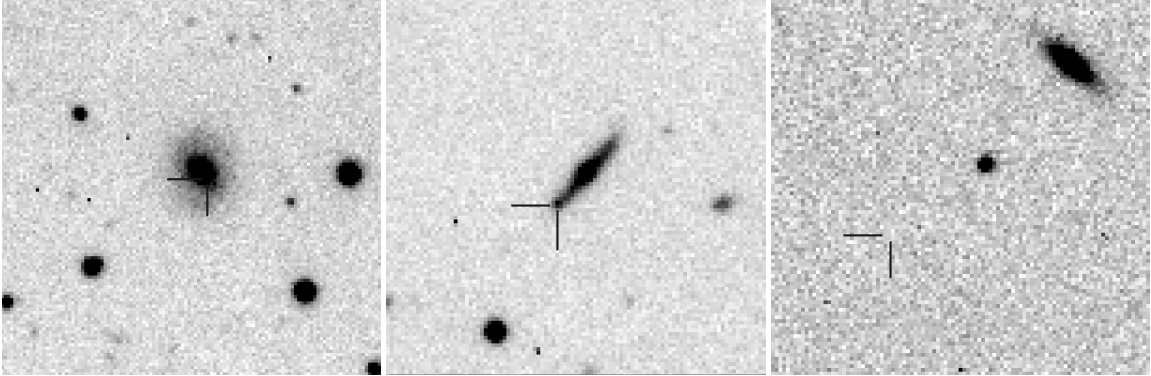
Figure 2: The diversity of short GRBs host galaxies. The early type host galaxy of GRB 050724 (Barthelmy et al. 2005; Malesani et al. 2007; left panel), the late-type host galaxy of GRB 071227 (D’Avanzo et al. 2009; central panel) and the host-less GRB 061201 (Stratta et al. 2007; Berger 2010; right panel). All images were obtained in the R -band with the ESO-VLT equipped with the FORS camera. Each box is 25'' \times 25'' wide. North is up and East is left. The solid lines mark the position of the optical afterglow.
