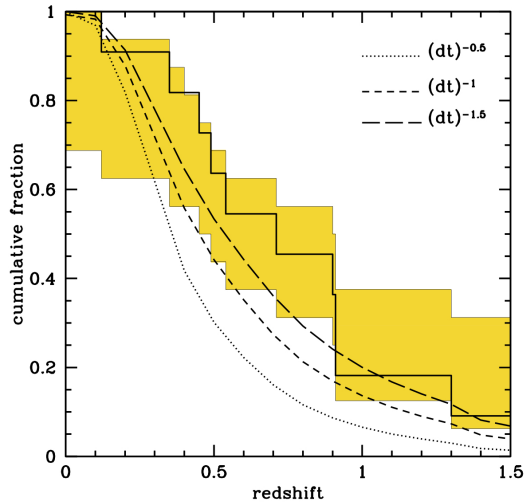
Figure 3: Redshift distribution of the S-BAT4 sample of SGRBs (from D’Avanzo et al. 2014). The shaded area takes into account the uncertainties due to the lack of redshift measurement for five bursts in the sample. Model results for n = -1.5 , -1 , and -0.5 are shown with the long-dashed, short-dashed and dotted line, respectively. In computing the expected redshift distribution for the different model we apply the same photon flux cut, P_{64} \geq 3.5 \text{ ph s}^{-1} \text{ cm}^{-2} in the Swift -BAT 15–150 keV band, used in the definition of the sample.
