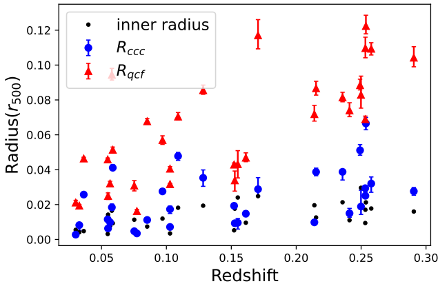
Fig. 6. Quenched cooling flow radius R_{qcf} (red) and the cool-core condensation radius R_{ccc} (blue) plotted versus redshift. The black dots show the size of the innermost bins, to visualize of how well we are able to resolve the inner regions compared with the R_{qcf} values.
