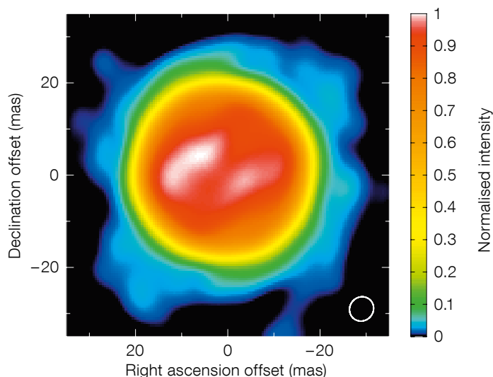
Figure 6. Velocity-resolved aperture synthesis imaging of the red supergiant Antares. This monochromatic image was obtained at the centre of the CO transition at 2.30665\ \mu\text{m} . AMBER's high spatial and spectral resolution allowed the observations to measure the "vigorous" motion above the complex red supergiant photosphere (adapted from Ohnaka, Weigelt & Hofmann, 2017).
