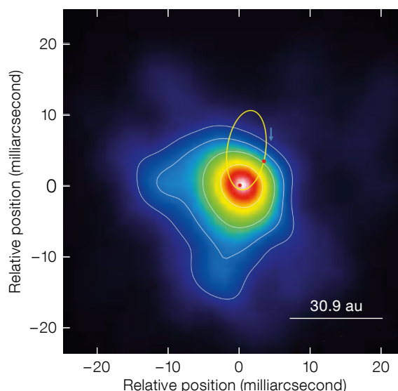
Figure 2. Aperture synthesis image of \eta Carinae in the Brackett \gamma H I transition at a radial velocity of -277 \text{ km s}^{-1} . The image shows both the dense stellar wind surrounding the primary star (red, yellow, and green regions) and the fan-shaped wind-wind collision zone (blue). The image field of view is 50 \times 50 milliarcseconds. Overlaid is a sketch of the orbit of the secondary star (adapted from Weigelt et al., 2016).
