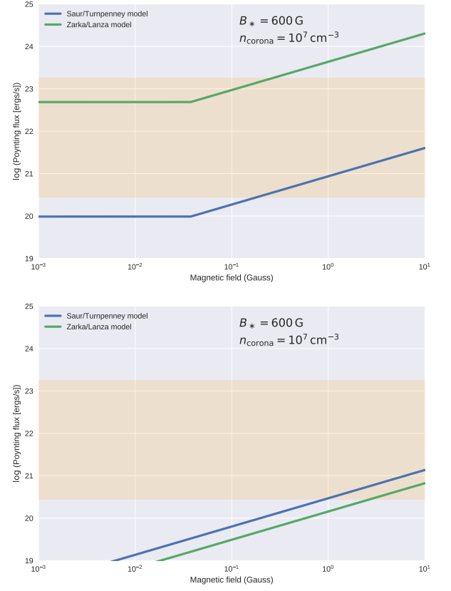
Fig. B.3. Comparison of theoretical expectations and observationally inferred values of the Poynting flux from sub-Alfvénic interaction in Proxima, as a function of the magnetic field of the planet Proxima b. Top: Open magnetic field; bottom: Closed magnetic field.
