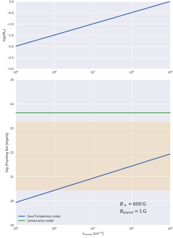
Fig. B.4. Comparison of theoretical expectations and observationally inferred values of the Poynting flux from sub-Alfvénic interaction in Proxima, as a function of density at the base of the stellar corona, for an open magnetic field geometry.
