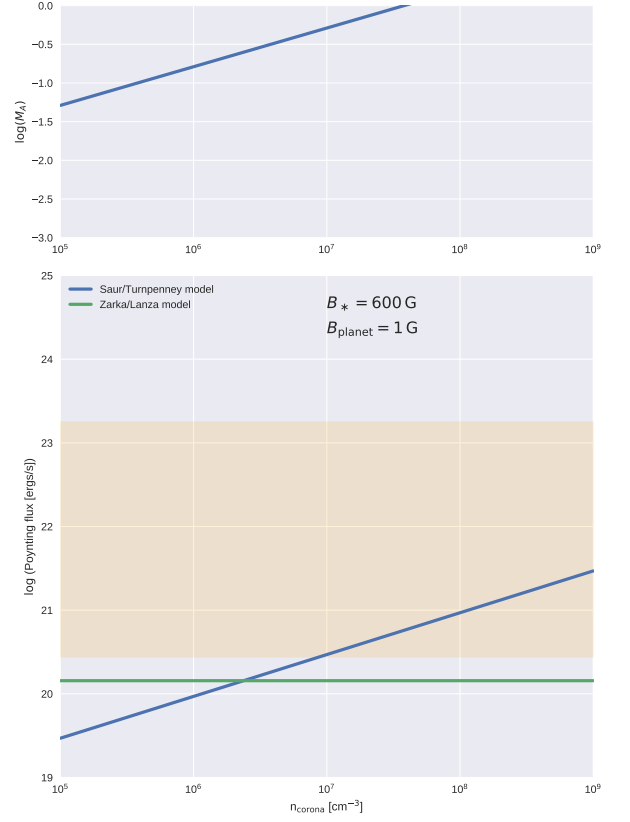
Fig. B.5. Same as in Fig. B.4, but for a closed magnetic field. The regime stops being sub-Alfvénic at the orbital distance of Proxima b for n_{\text{corona}} \approx 3.8 \times 10^7 \text{ cm}^{-3} , corresponding to a density of about 7000 \text{cm}^{-3} at the orbital position of Proxima b.
