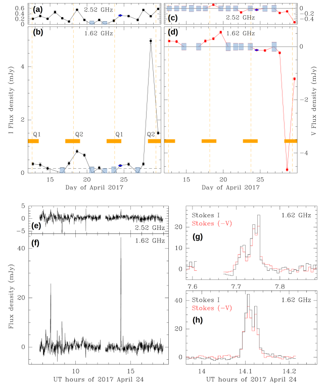
Fig. 2. Time evolution of flux density in Proxima. Variation of total (Stokes I; panels a and b) and circularly polarized (Stokes V; panels c and d) flux density as a function of time during our ATCA observing campaign. For each observing session, we averaged the data over a bandwidth of 400 MHz and 1 GHz centered at 1.62 GHz [wavelength \approx 18.5 \text{ cm} ; (b,d)] and 2.52 GHz [ \approx 11.9 \text{ cm} ; (a,c)], respectively. 1\sigma uncertainties are plotted as vertical lines for each data point, and blue shaded rectangles mark 3\sigma upper limits for non-detections (in the case of Stokes V, they correspond to upper limits to the absolute value of the flux density). The duration of the observation on April 24 (12 hours) is represented with a horizontal blue bar, while the observing time of the other days ( \sim 2 hours) is smaller than the symbol size of data points. Dashed orange lines show the quadratures, Q1 and Q2, of Proxima b, with the horizontal orange bars indicating the uncertainty in the determination of the epoch of the quadratures (see main text for details). The horizontal dashed line in the plot of Stokes I at 1.62 GHz (b) corresponds to a flux density of 0.174 \pm 0.038 \text{ mJy} , obtained by averaging together the data over the five observing sessions where the source was not detected individually at that frequency. No map could be obtained at low frequency on April 15, due to an insufficient number of unflagged visibilities. (e–f) Variation of Stokes I during 2017 April 24 for data averaged over 20 s intervals. Two short-duration flares are evident at 1.62 GHz (f). (g–h) Temporal close-up of the two flares. Black and red lines correspond to Stokes I and V, respectively. The sign of Stokes V has been reversed for better visualization.
