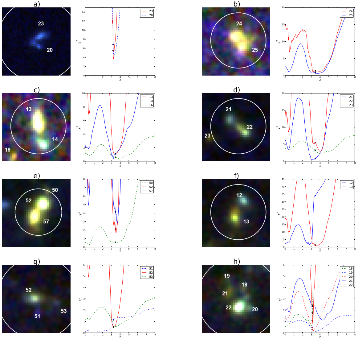
Fig. A.1. BVI colour images ( left panels ) and \chi^2 function versus photometric redshift ( right panels ). a) Object ID_CANDELS=6839 ( z = 3.208 ): kept in the clean sample. It is composed of two clumps (numbers 23 and 20). The upper is brighter than the lower one. The white circle in the left panel has a radius equal to the PSF full width at half maximum of the ground-based narrow-band image, sampling the LyC at z = 3.208 . The solid (dashed) line in the right panel corresponds to the brighter (fainter) clump, while the blue (red) dot indicates the \chi^2 of the SED fit derived by fixing the value of the redshift to the spectroscopic one. b) Object ID_CANDELS=4022 ( z = 3.466 ): kept . The two solid lines in the right panel show that the two clumps (numbers 24 and 25) are equally bright. c) Object ID_CANDELS=3768 ( z = 3.468 ): kept . The red and blue dots overlap. d) Object ID_CANDELS=3325 ( z = 3.473 ): kept . e) Object ID_CANDELS=15 220 ( z = 3.469 ): kept . The two solid lines in the right panel show that the two clumps are equally bright (numbers 52 and 57). f) Object ID_CANDELS=7645 ( z = 3.478 ): removed . g) Object ID_CANDELS=17 905 ( z = 3.242 ): removed . In the right panel , the red and green dots overlap. h) Object ID_CANDELS=23 527 ( z = 3.116 ): removed . It is composed of five clumps. The two reddest ones have a broad \chi^2 function. The main component (number 22) is perfectly fitted at the spectroscopic redshift.
