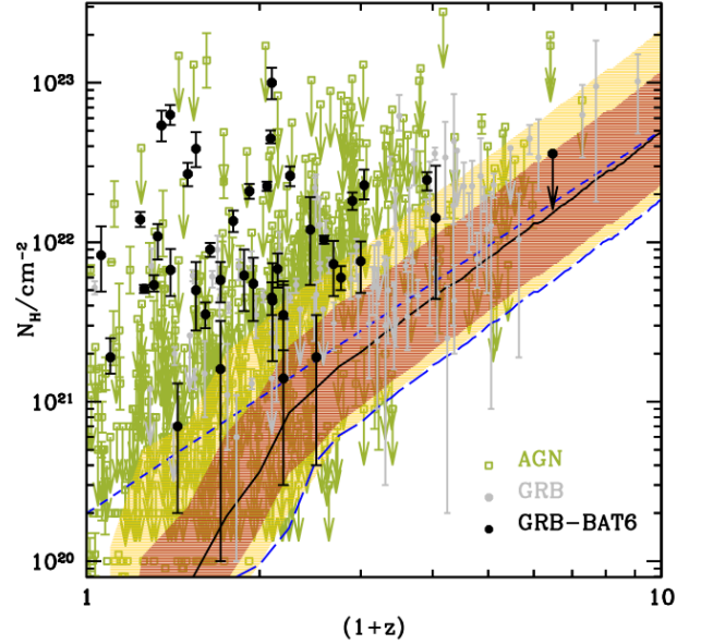
Fig. 2. Distribution of equivalent hydrogen column densities, N_{\text{H}} , with redshift as measured for different sources: GRBs with measured redshift (grey dots), bright GRBs in a redshift complete sample (black dots), and AGN (green squares). Error bars are at 1\sigma confidence level. The long dashed curve represents the LOS with the lowest absorption, i.e. with no absorbers with density contrast \Delta > 100 , and constant metallicity ( Z \sim 0.03 Z_{\odot} ). This curve was obtained from cosmological simulations, summing up the contribution by each cell, with an absorbing column density weighted for its effective (temperature-dependent) value. The results for a physically motivated model of SN winds (momentum-driven model by Oppenheimer et al. [2012]) are shown by the solid line (median of LOS distribution) and corresponding shaded areas (68% and 90% of LOS, respectively). The short dashed line corresponds to the median LOS with \log N_{\text{H}} = 20.3 \pm 0.1 ( 1\sigma confidence level) obtained considering constant metallicity ( Z = 0.3 \pm 0.1 Z_{\odot} ) in absorbers with 100 < \Delta < 1000 .
