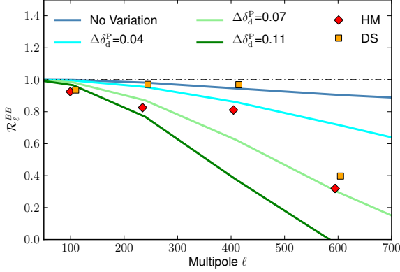
Fig. 5. Illustration of the correlation ratio modelled with Gaussian spatial variations of the polarized dust spectral index, in LR42 as in Fig. 2. The HM and DS Planck measurements are shown as diamonds and squares, respectively. The model is plotted for four values of \Delta\delta_d^p , which is defined as the standard deviation of the Gaussian realization of the spectral index after smoothing at 1^\circ . The first model, with \Delta\delta_d^p = 0 , is that described in Sect. 3.2.
