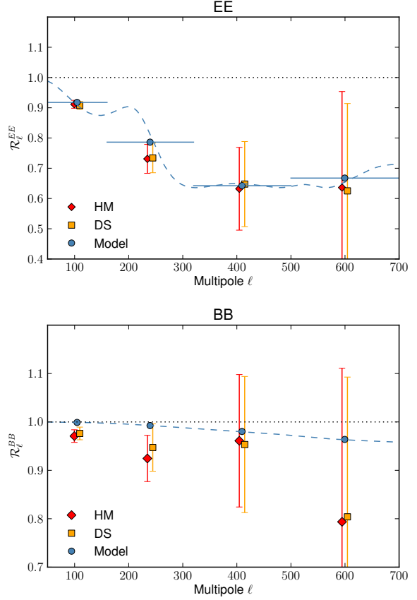
Fig. 2. Dust polarization correlation ratios \mathcal{R}_\ell^{EE} (top panel) and \mathcal{R}_\ell^{BB} (bottom panel) between 217 and 353 GHz, computed on the LR63 region. The correlation ratios determined from the detector-set data (DS) splits are displayed as yellow squares and the ratios computed from the half-mission (HM) splits are displayed as red diamonds. The correlation ratio expectations for the model described in Eq. (5) are displayed as blue dashed lines (blue circles when binned as the data). Horizontal blue segments in the top panel represent the range of the \ell bins. The uncertainties have been estimated as the median absolute deviation over a set of 1 000 simulations (see Sect. 2.3) of CMB, dust, and Gaussian noise.
