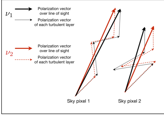
Fig. 7. Illustration of the decomposition of the line of sight polarization pseudo-vector into a random walk process through four turbulent layers. This is shown for two neighbouring pixels at two frequencies, \nu_1 and \nu_2 . The integrated polarization pseudo-vectors are affected by the polarization angle fluctuations, leading to a decorrelation between the two frequencies.
