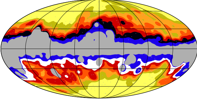
Fig. 1. Masks and complementary science regions that retain fractional coverage of the sky, f_{\text{sky}} , from 0.8 to 0.2 (see details in Sect. 2.2). The grey is the CO mask, whose complement is a selected region with f_{\text{sky}} = 0.8 . In increments of f_{\text{sky}} = 0.1 , the retained regions can be identified by the colours yellow (0.3) to blue (0.8), inclusively. The LR63N and LR63S regions are displayed in black and white, respectively, and the LR63 region is the union of the two. Also shown is the (unapodized) point source mask used.
