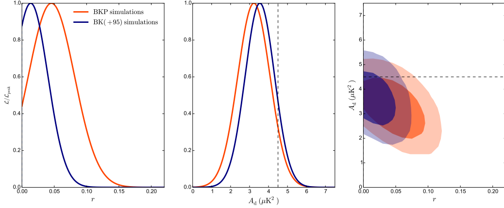
Fig. 4. C_\ell^{BB} spectra likelihood posteriors on the r and A_d parameters derived from the simulations of the BICEP2-Keck and Planck 353-GHz data, using: 150- and 353-GHz channels (BKP, red); and 95-, 150- and 353-GHz channels (BK(+95), blue). The 1D posteriors of r (marginalized over \beta_d^p and A_d ) and of A_d (marginalized over \beta_d^p and r ) are displayed in the left and middle panels (blue and red lines, respectively). The input value in our simulations for the dust amplitude at 353 GHz ( 4.5 \mu\text{K}^2 at \ell = 80 ) is indicated as a dashed line. The 2D posterior marginalized over \beta_d^p is presented in the right panel (68 % in darker shading and 95 % in lighter shading).
