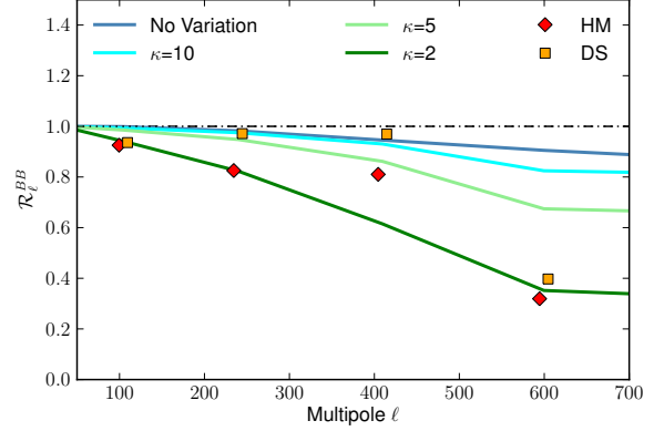
Fig. 6. Like Fig. 5, but illustrating the correlation ratio modelled with Gaussian spatial variations of the polarization angle. The model is plotted for four values of \kappa , which sets the level of the circular normal distribution for polarization angle, analogous to 1/\sigma^2 for the normal distribution.
