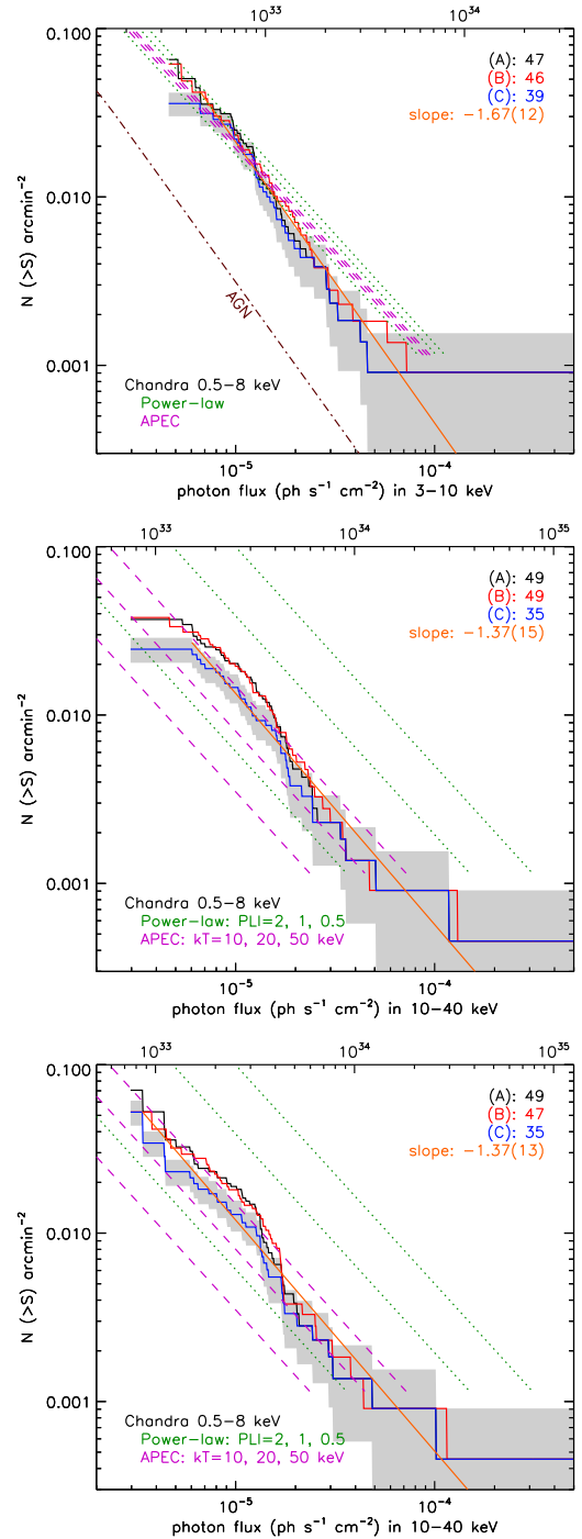
Figure 14. Comparison of the NuSTAR 3–10 keV (top) and 10–40 keV logN–logS distributions (middle and bottom) with the Chandra 0.5–8 keV logN–logS distribution. The top two panels use the model-based flux estimation, and the bottom panel use the non-parametric flux estimation (Sections 4.4 and 6.4). (A-black) The group-1 and 2 sources with the first aperture sets (see Section 4.1), (B-red) with the second aperture sets and (C-blue) the group-1 sources with the first aperture sets. The gray region shows the statistical errors for (C) and the (yellow) solid line is the best fit for (C). The (green) dotted and (magenta) dashed lines show the Chandra 0.5–8 keV logN–logS distribution from M09: green dotted lines are for power-law models with \Gamma = 2, 1 and 0.5 (from bottom to top) and magenta dashed lines are for APEC with kT = 10, 20 and 50 keV (from bottom to top). The brown dashed-dot line in the top panel is AGN (Kim et al. 2007).
