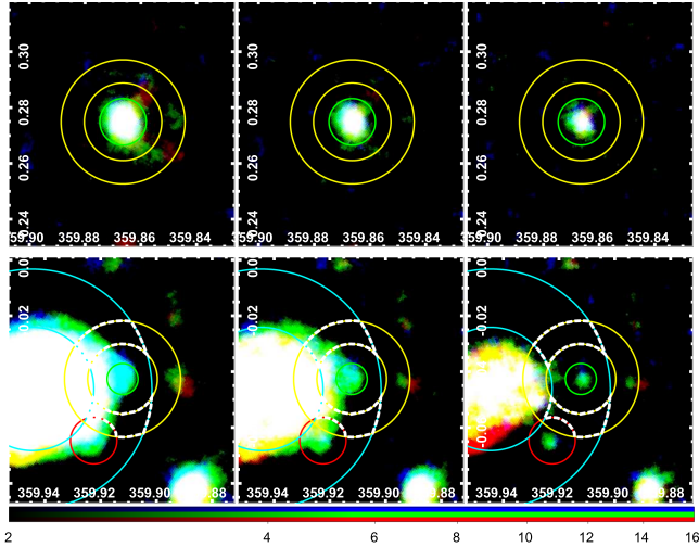
Figure 7. Example aperture selections for photometry overlaid in the trial maps centered around NGP 3 (top) and NGP 34 (bottom). From left to right, the trial maps for 30%, 20% and 15% PSF enclosures for source cells are shown to illustrate the scales of the source and surrounding diffuse emission relative to the aperture selections. In the case of NGP 34, the intersection of the two annuli (yellow and cyan) excluding the neighboring source (red) is used for the background aperture (the dashed lines). The colors are scaled with the logarithmic values ( X ) of trial numbers ( 10^X ).
