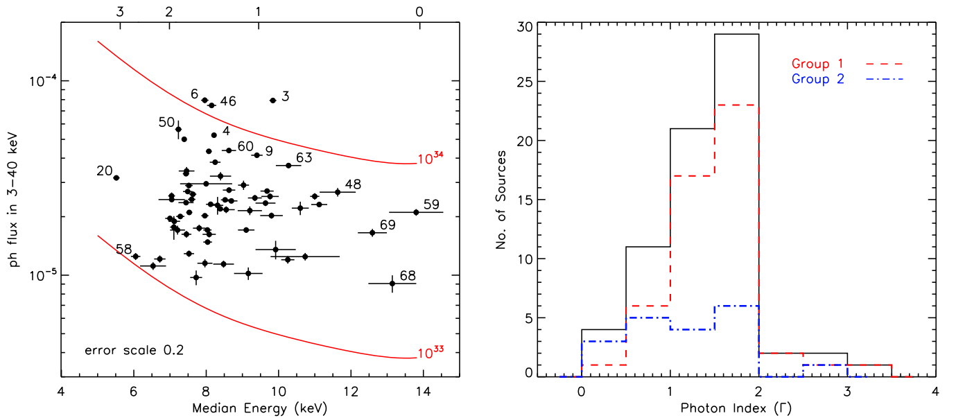
Figure 9. Scatter plot of photon flux vs. median energy of the NuSTAR sources (left) and their equivalent photon index distribution (right). The top x-axis on the left panel shows the equivalent photon indices for an absorbed power-law model with N_H = 6 \times 10^{22} \text{ cm}^{-2} (Section 4.3). The two lines show the iso-luminosity tracks for L_X = 10^{33} and 10^{34} \text{ erg s}^{-1} at 8 kpc in the 3–40 keV band. The error bars are scaled down to 20% of the original values for easy viewing. The red, blue and black histograms show group-1, 2 sources and the sum of the two, respectively.
