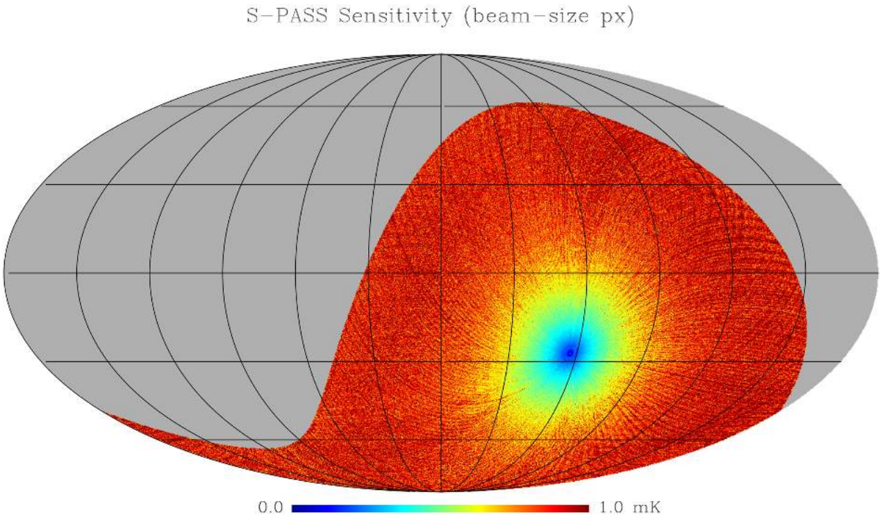
Figure 19. S-PASS sensitivity map on the beam-size scale. The map is in Mollweide projection, Galactic coordinates, with the Galactic centre at the centre and longitude increasing leftward.
