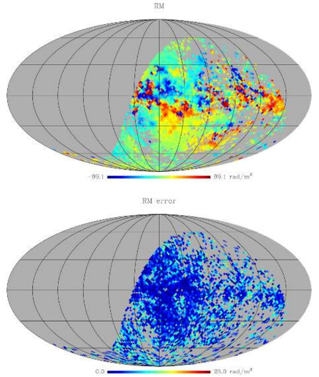
Figure 31. Top: map of RM obtained combining best-fitting S-PASS (2.3 GHz), WMAP (22.8 GHz) and Planck (28.4 GHz) polarization angle maps. Bottom: RM errors ( 1-\sigma ) from the fit procedure.
