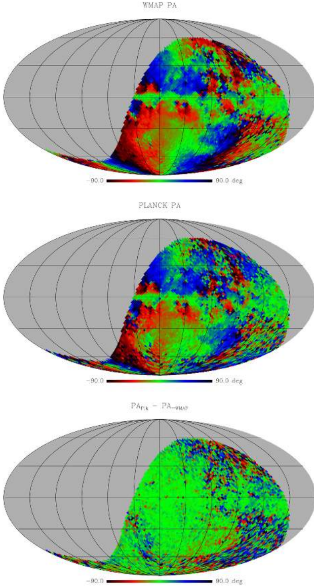
Figure 30. WMAP polarization angle map at 23 GHz (top), Planck map at 30 GHz (middle) and their difference (bottom).
