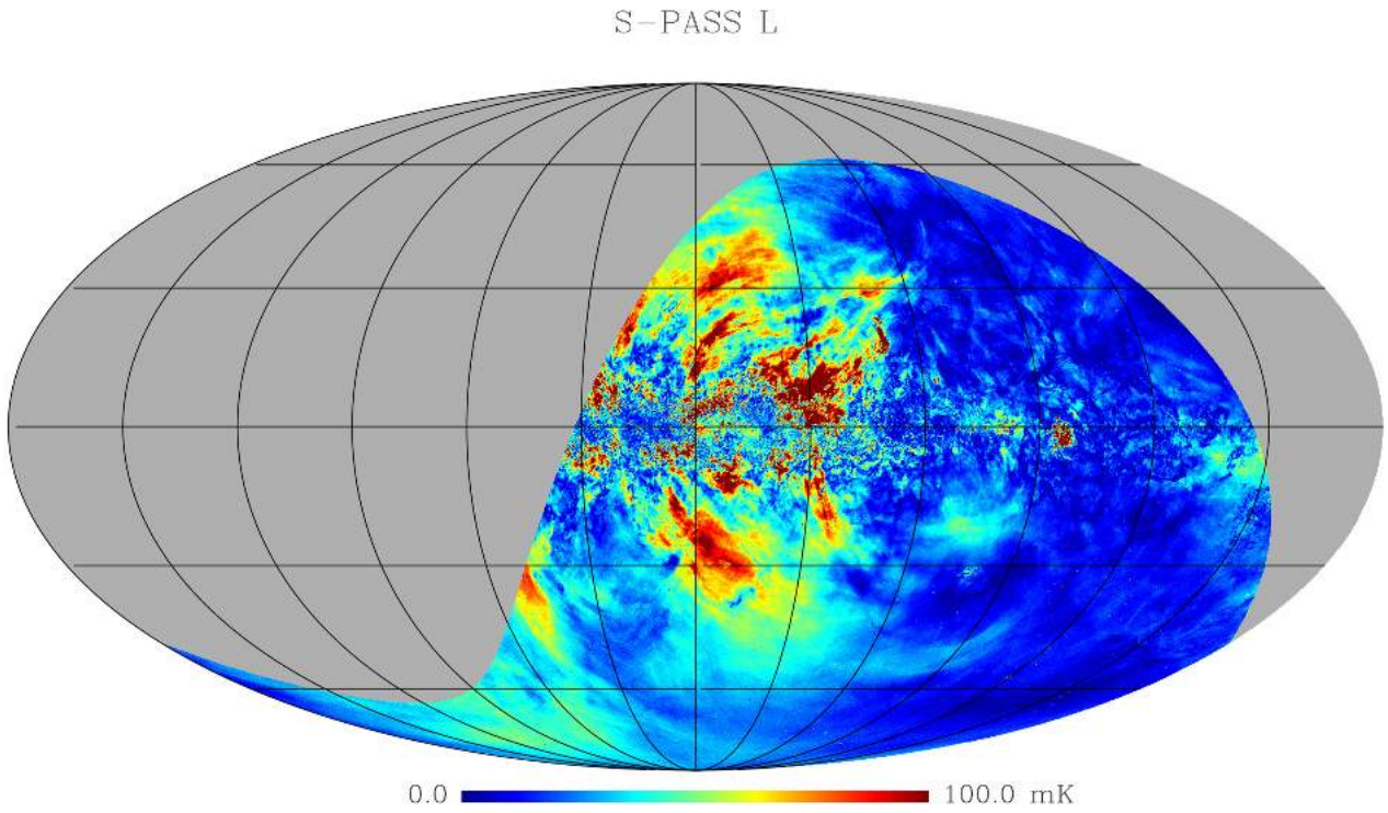
Figure 18. S-PASS map of linear polarized intensity L . The map is in Mollweide projection, Galactic coordinates, with the Galactic centre at the centre and longitude increasing leftward.
