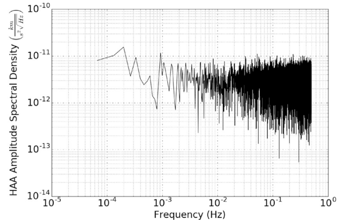
Fig. 4. HAA random noise amplitude spectral density.
