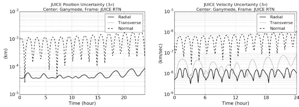
Fig. 7. JUICE reconstructed position and velocity during a 1-day arc as result of 3GM precise orbit determination. The position is expressed in km and the velocity in km/s in the JUICE RTN (radial, transverse, normal) frame pointing towards Ganymede.
