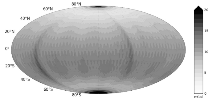
Fig. 6. Hammer-Aitoff projection map of Ganymede's gravity field uncertainty.
