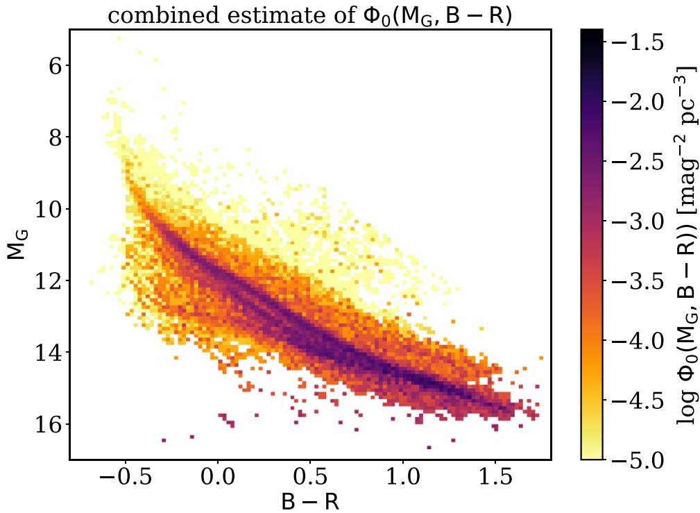
Figure 10. Estimate of the WD luminosity–color density (LCF) from a combination of the previous estimates. The high-density regions were estimated using the \bar{S}/\bar{N}_{\varpi, \min} > 80 sample to take full advantage of the precise parallaxes for the sharp features in the diagram. The other parts were estimated from the \bar{S}/\bar{N}_{\varpi, \min} > 20 sample, and finally from the \bar{S}/\bar{N}_{\varpi, \min} > 5 sample that had been calculated on a coarser grid; these latter two steps reduce sampling noise in the low-density parts of the distribution.
