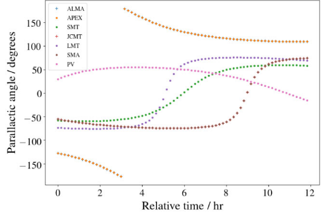
Figure 6. Evolution of the parallactic angles of EHT 2017 array stations over 12-h in the direction of M87.
