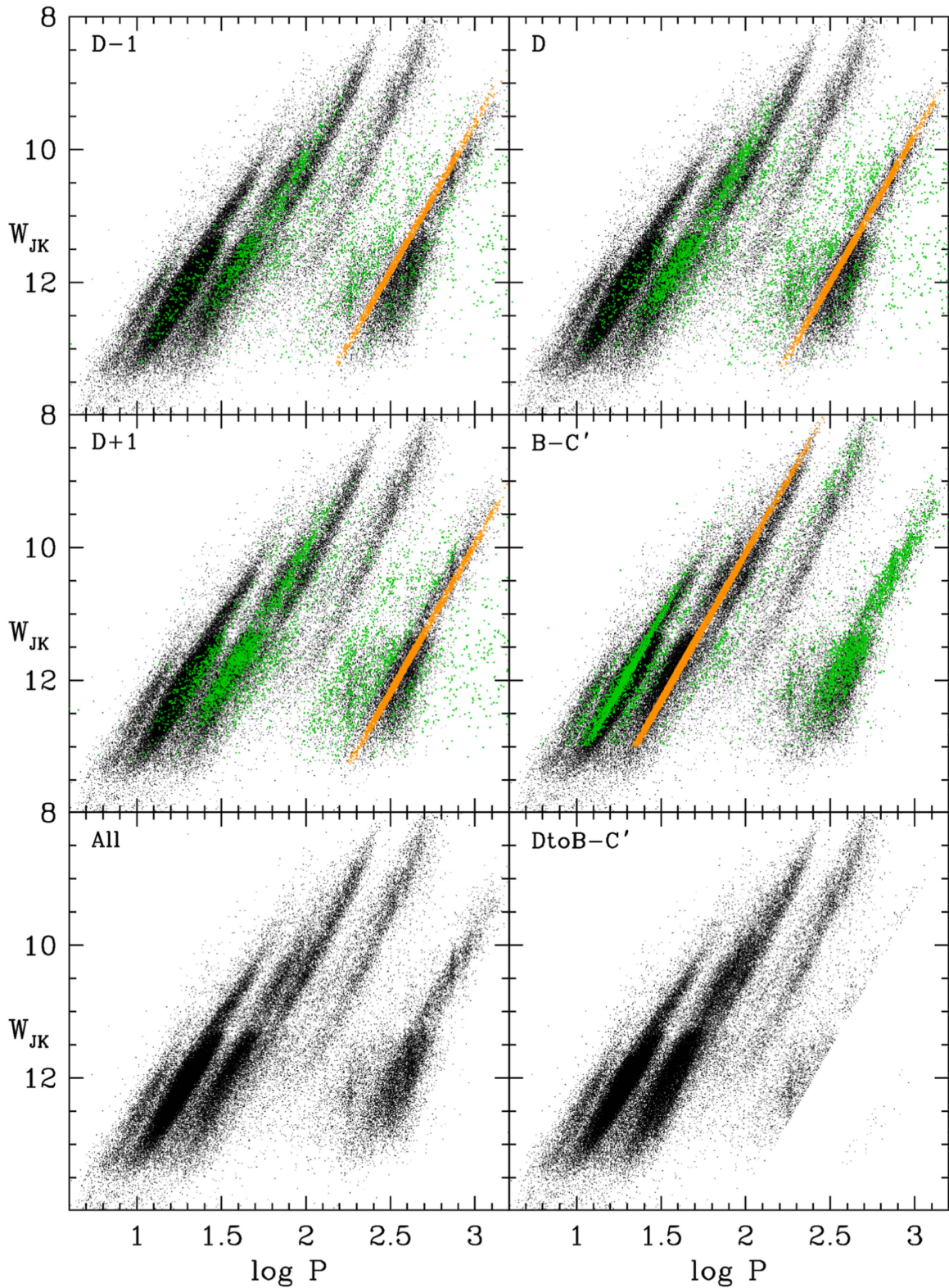
Figure 6. Similar to Figure 4. In panels (D-1), (D), and (D+1), the channels are placed in sequence D. In panel (B-C'), the meanings of the orange and green points are reversed so that the orange points correspond to secondary or tertiary periods and the green points are the primary periods of the stars marked with orange points. In panel (All), the raw OGLE III data is plotted. In panel (D to B-C'), the sequence D variables have been shifted to a position lying between sequences B and C', as described in the text.
