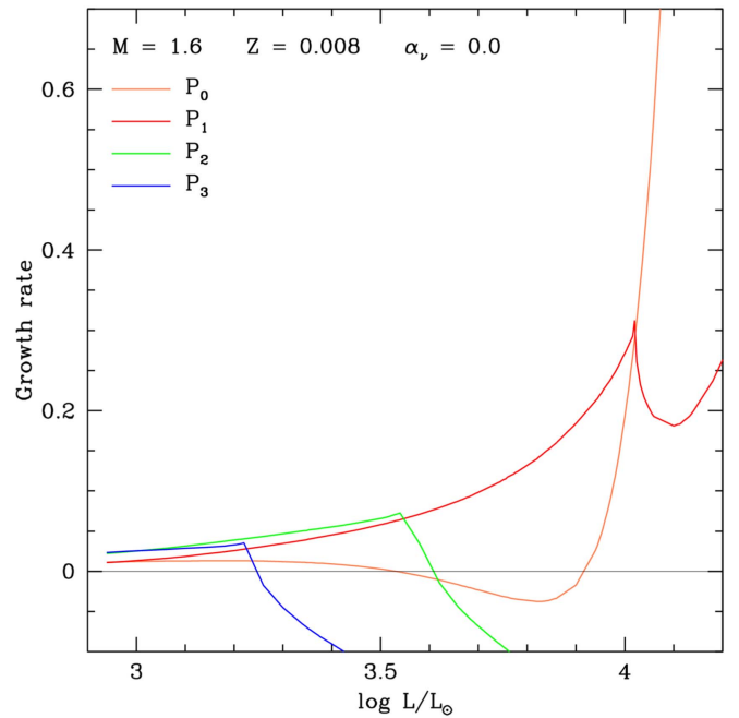
Figure 5. Growth rate of the first four radial pulsation modes in a 1.6 M_{\odot} star as a function of luminosity. The metallicity is LMC-like ( Z = 0.008 ) and turbulent viscosity has been neglected. See Wood & Olivier (2014) for details of the modeling.
