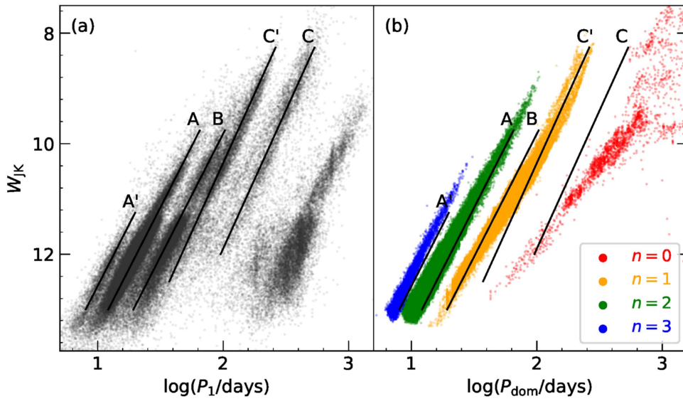
Figure 1. Observed primary periods (panel (a)) are compared to theoretically dominant periods obtained from radial, linear, nonadiabatic models (panel (b)). Different colors represent periods of different modes: red for fundamental mode, orange for 1O, green for 2O mode, and blue for 3O mode. Solid lines provide a visual aid to identify the approximate location and slope of observed sequences.
