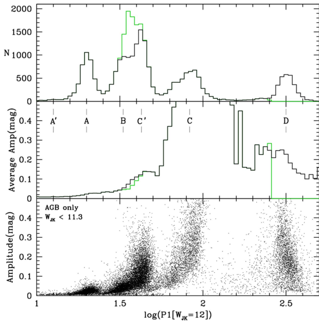
Figure 7. Bottom panel: pulsation amplitude of individual AGB stars in the OGLE III catalog plotted against \log(P_1[W_{JK}=12]) . The selected AGB stars have W_{JK} < 11.3 . Middle panel: the average amplitude of the AGB stars in bins of width 0.025 in \log(P_1[W_{JK}=12]) . Top panel: the numbers of stars in the bins. The positions of the PL sequences are shown in the middle panel. Black lines and points are plotted when the stars have values of \log(P_1[W_{JK}=12]) in the OGLE III catalog. The green lines in the top panel are plotted when \log(P_1[W_{JK}=12]) values for all stars in sequence D have been shifted to a new value between sequences B and C', as described in the text. The green lines in the middle panel are plotted when only the 40% of sequence D stars with a secondary or tertiary period between sequences B and C' have been shifted.
