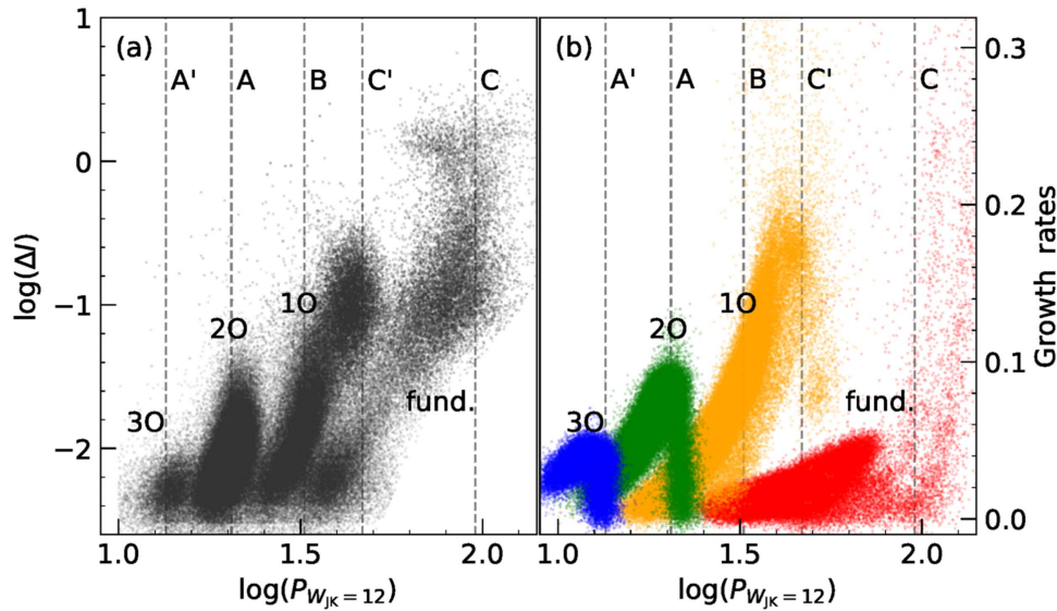
Figure 2. Panel (a): logarithm of observed I -band amplitudes, for all three periods of stars in the OGLE3 catalog, as a function of \log(P_{W_{JK}=12}) . The distinct PAL relations are labelled with the corresponding mode according to the interpretation provided here (see the text). Periods on sequence D and longer than sequence C have been ignored, as they are not related to the normal modes of pulsation (see Section 3.1). Panel (b): theoretical growth rates for all excited modes up to the 3O, labelled and color coded according to their radial order as in Figure 1. Vertical dashed lines in the background of both panels approximately identify the center of the PL sequences.
