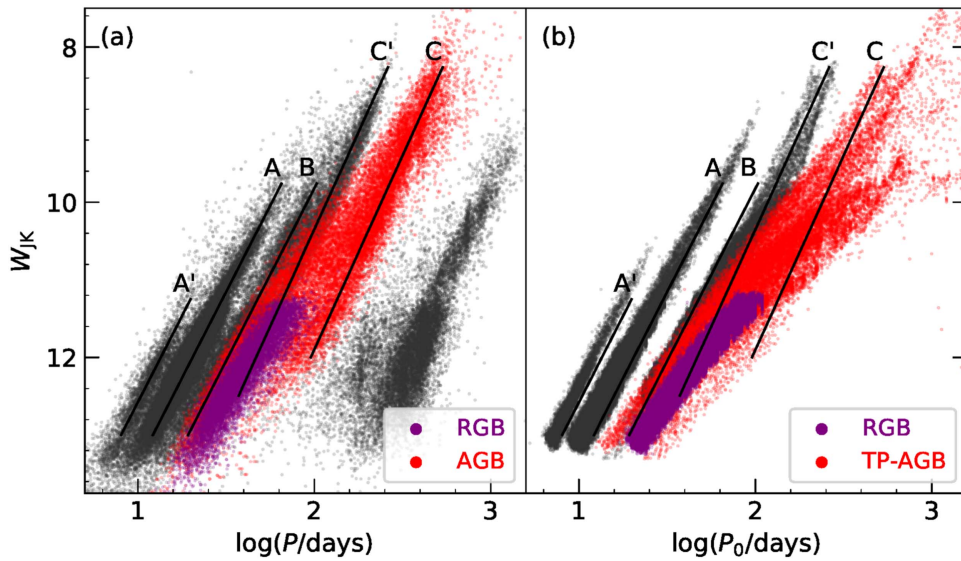
Figure 3. Panel (a): each star in the OGLE3 Catalog has three observed periods: primary, secondary, and tertiary. Here, all of them are shown, provided that they belong to the fourth amplitude group in Figure 2 (labelled “fund”). They are shown as red or purple points if classified, respectively, as AGB or RGB stars (according to the OGLE evolutionary classification as in Soszyński et al. 2004). As a reference, all primary periods are shown in the background as dark points (same as Figure 1). Panel (b): theoretical fundamental mode periods, regardless of their growth rates, shown in red if they belong to TP-AGB models and in purple if they belong to RGB models. Dominant overtone modes are shown as dark points in the background for reference.
