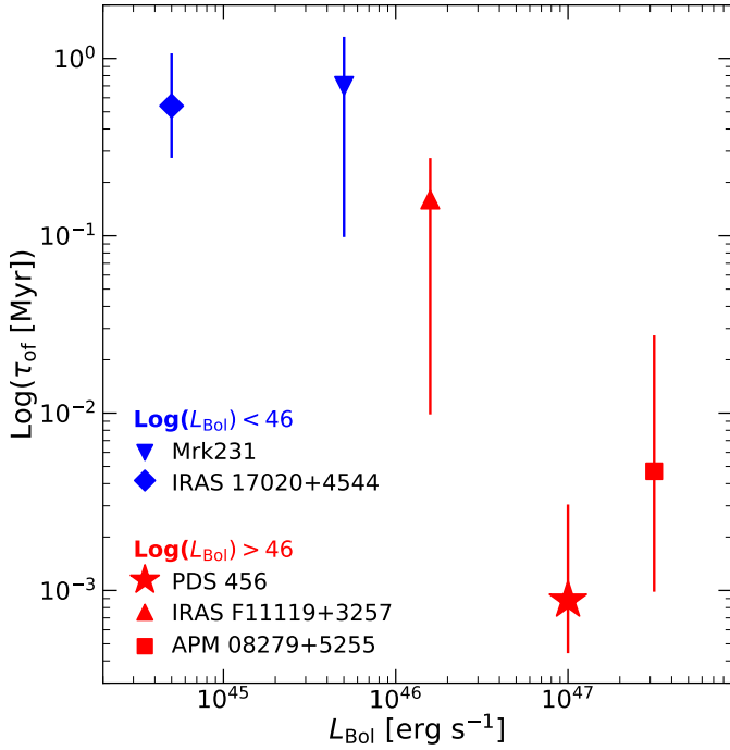
Fig. 10. \tau_{\text{of}} = E_{\text{of}}/\dot{E}_{\text{UFO}} as a function of L_{\text{Bol}} for PDS 456 and a compilation of AGNs as in Fig. 9. E_{\text{of}} is computed under the assumption that the bulk of the outflowing gas mass is in the molecular phase. Blue (red) symbols correspond to AGNs with L_{\text{Bol}} < 10^{46} \text{ erg s}^{-1} ( L_{\text{Bol}} > 10^{46} \text{ erg s}^{-1} ).
