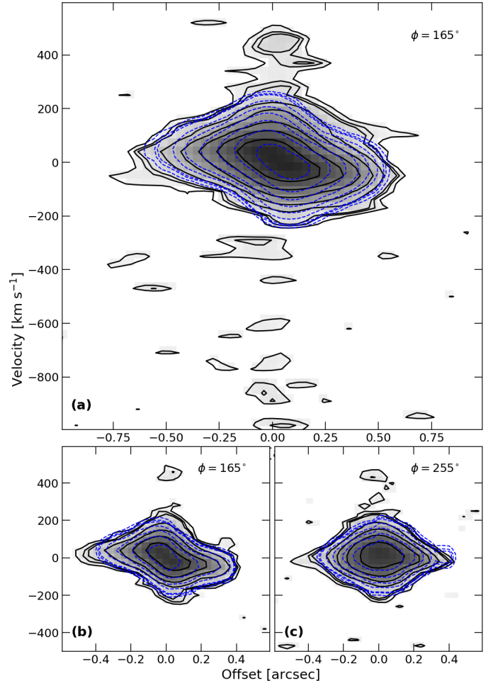
Fig. 5. Panel a: position–velocity diagram, extracted from a 0.3 \text{ arcsec} slit centred on the QSO location along the major kinematic axis (see Fig. 4a) corresponding to a PA of 165^\circ (measured anti-clockwise from north). Black contours refer to the [2, 3, 4, \dots, 2^n]\sigma significance level of the CO(3–2) emission, with \sigma = 0.083 \text{ mJy beam}^{-1} and n > 2 . The contours associated with the best-fit 3\text{D} BAROLO model of the kinematics are also shown by the blue contours. Panels b and c: zoom-in of the velocity range v \in [-500, +600] \text{ km s}^{-1} with increased angular resolution ( 0.16 \times 0.19 \text{ arcsec}^2 ), extracted along and perpendicular to the major kinematic axis, respectively. Contours are as in the top panel, with \sigma = 0.16 \text{ mJy beam}^{-1} .
