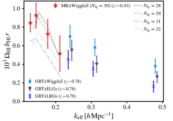
Figure 7. Constraints on \Omega_{\text{HI}} b_{\text{HI}} r measured at different effective scales k_{\text{eff}} , achieved by removing low- k data points from the cross-power spectrum, the data-points for each case are therefore not independent. The results for this paper are shown in red-stars using an N_{\text{fg}} = 30 PCA clean and the four grey lines show results from different values of N_{\text{fg}} . For comparison we also plot the recent results from GBT cross-correlations (W22).
