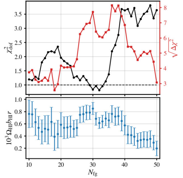
Figure 6. Sensitivity of results to foreground cleaning. Top panel, left-axis, and black-dot data show the reduced \chi^2 for each foreground cleaned cross-power spectra relative to its best-fitting model. Top panel, right-axis, and red-square data show the detection significance for the cross-power spectra relative to a null model. Bottom panel shows the variation in the best-fitting \Omega_{\text{HI}} b_{\text{HI}} r for each N_{\text{fg}} case, from a least-squares fit to the cross-power spectrum amplitude.
