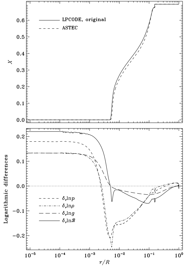
Fig. F.4. Top panel: hydrogen abundance in the ASTEC (dashed) and the original LPCODE 2.5 M_\odot , 10 R_\odot solar-calibrated models. Bottom panel: differences \delta_r \ln p (dashed), \delta_r \ln \rho (dot-dashed), \delta_r \ln g (long dashed) and \delta_r \ln \mathcal{B} (solid) between the ASTEC and the original LPCODE 2.5 M_\odot , 10 R_\odot models, in the sense (LPCODE) – (ASTEC).
