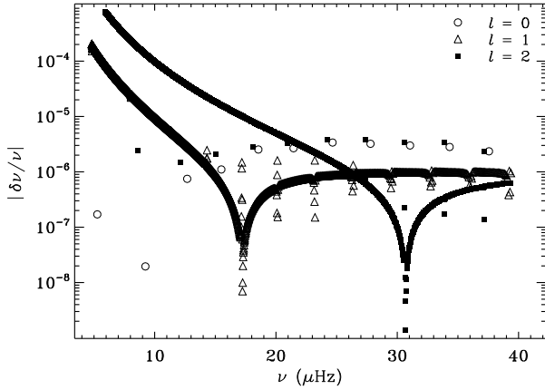
Fig. A.2. Absolute value of relative frequency differences, at fixed radial order, between computations with 38 400 and 19 200 points for the 1.0 M_{\odot} , 12 M_{\odot} case.
