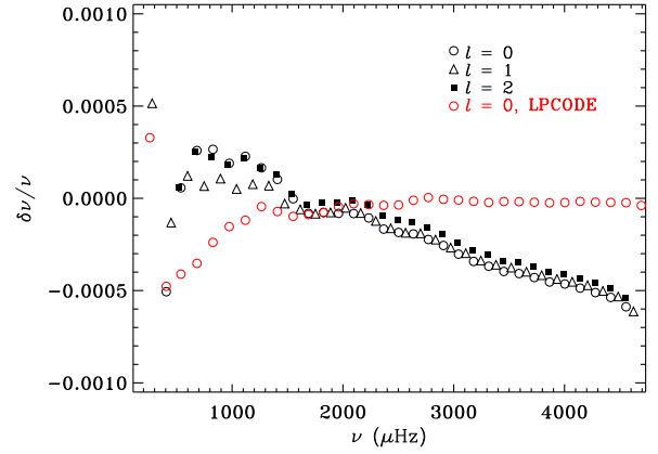
Fig. D.2. Relative frequency differences for the (1 M_{\odot}, 1 R_{\odot}) solar-calibrated case between MESA and ASTEC, in the sense (MESA) – (ASTEC), for l = 0 (open circles), l = 1 (open triangles) and l = 2 (filled squares) in black. The differences are evaluated at fixed radial order. The red circles show corresponding results for radial modes in the LPCODE model.
