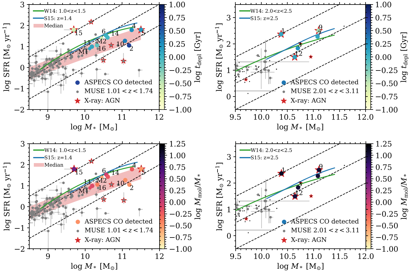
Figure 12. Stellar mass ( M_* ) vs. SFR for the galaxies at 1 < z < 1.7 (left) and 2 < z < 3.1 (right). The ASPECS-LP detections from the full and prior-based search are represented by the larger and smaller circles respectively. The gray and black points show the MUSE and photometric reference samples of galaxies, respectively. Red stars indicate X-ray sources identified as AGN from Luo et al. (2017). The color in the different panels denotes the change in depletion time ( t_{\text{depl}} = M_{\text{mol}}/\text{SFR} ; top) and molecular-to-stellar mass ratio ( M_{\text{mol}}/M_* ; bottom). The green and blue solid curves denote the MS relationships from, respectively, Whitaker et al. (2014) and Schreiber et al. (2015). The red band shows \pm 0.3 dex around a polynomial fit to the running median of all galaxies in the panel. Lines of constant s\text{SFR} (0.1, 1, and 10 \text{Gyr}^{-1} ) are shown black and dashed. The gas fraction and depletion time vary systematically in galaxies across the main sequence.
