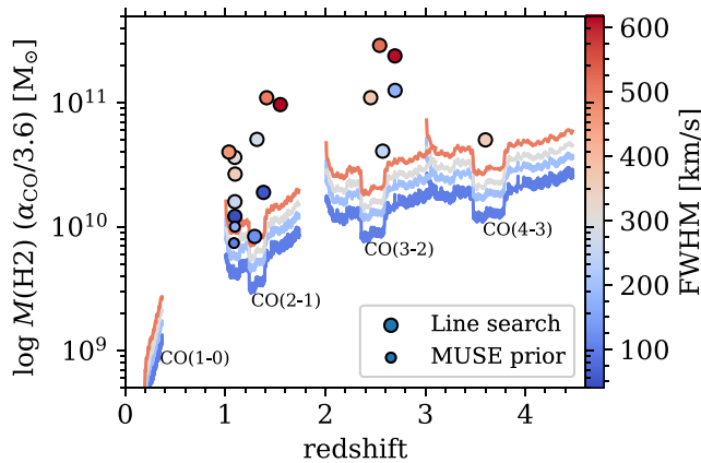
Figure 9. The 5\sigma molecular gas mass detection limit of ASPECS-LP as a function of redshift and CO line full width at half maximum (FWHM), assuming \alpha_{\text{CO}} = 3.6 and Daddi et al. (2015) excitation (see Section 4.3). The sensitivity varies with redshift and increases with the square root of the decreasing line width at fixed luminosity, indicated by the color. The points indicate the ASPECS-LP blind and prior-based sources, which are detected both in the deeper and shallower parts of the sensitivity curve.
