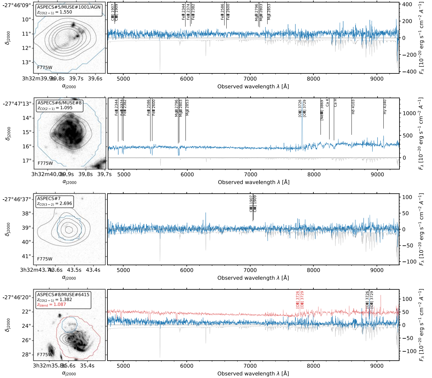
Figure 14. Continuation of Figure 13. We show spectrum of the complete system of spiral galaxies at ASPECS-LP.3mm.08 in red (scaled down by a factor of 10), to make the faint [O II] \lambda 3726, 3729 line matching the CO(2–1) redshift visible. The spectrum for ASPECS-LP.3mm.08 itself is shown in blue (extracted only over a part of the spiral arm). Note the foreground source is independently detected in CO(2–1) as ASPECS-LP-MP.3mm.02 and the fully annotated spectrum for this source is shown in Figure 15.
