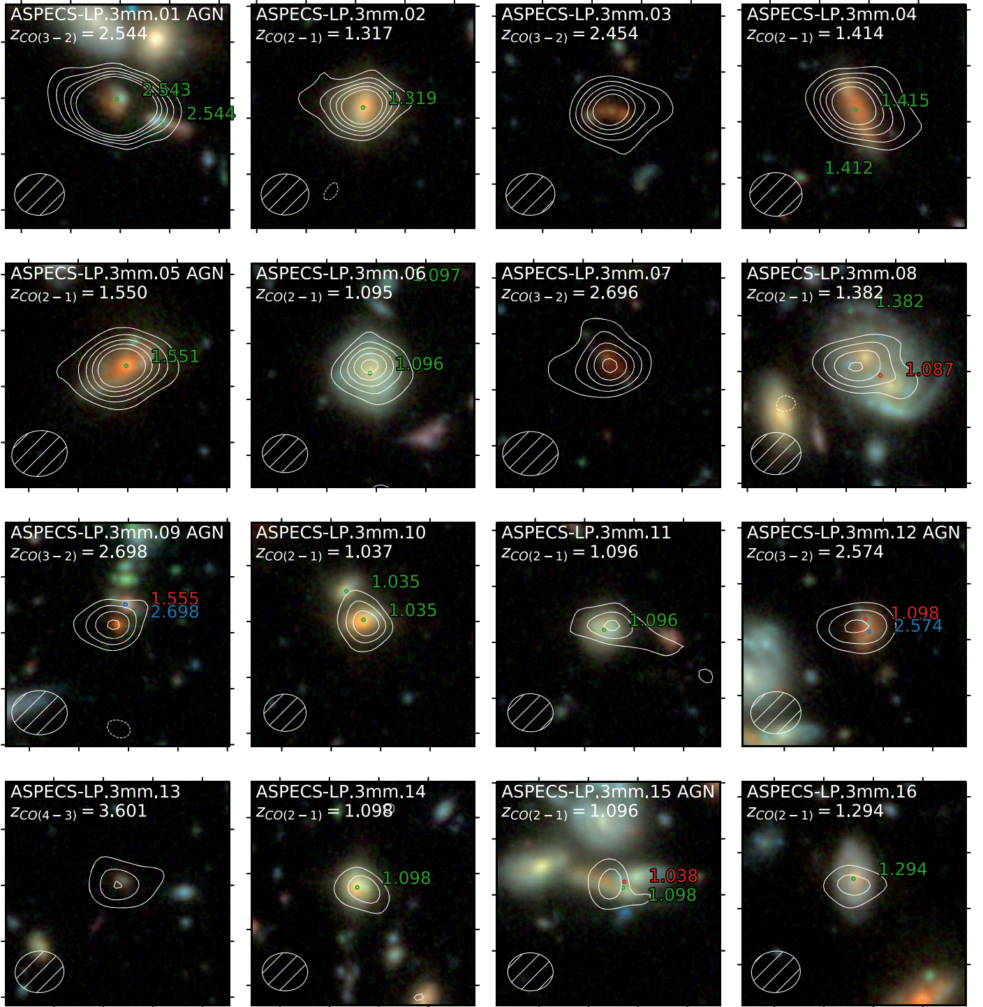
Figure 2. HST RGB cutouts (F160W, F125W, and F105W) of the 16 CO line detections from the line search, all revealing an optical/NIR counterpart. Each panel is 8'' \times 8'' centered around the CO emission (corrected astrometry; Section 2.1). The white contours indicate the CO signal from \pm[3, \dots, 11]\sigma in steps of 2\sigma . The ALMA beam is indicated in the bottom left corner. Galaxies with a spectroscopic redshift from MUSE (Inami et al. 2017) matching the CO signal are labeled in green (and red if not matching); spectroscopic redshifts in blue are newly determined in this paper. Of the 16 galaxies, 12 match closely to a redshift from MUSE (including ASPECS-LP.3mm.08, discussed in Appendix A and Decarli et al. 2016). ASPECS-LP.3mm.03, 3mm.07, and 3mm.09 have m_{F775W} > 27 , which is too faint for a direct absorption line redshift from MUSE (but are independently confirmed). For ASPECS-LP.3mm.09 we do find UV absorption features matching the CO(3–2) in the galaxy slightly to the north. A new absorption line redshift is found for ASPECS-LP.3mm.12 (see Figure 18). The photometric redshift and absence of lower- z spectral features indicate ASPECS-LP.3mm.13 being at z = 3.601 .
