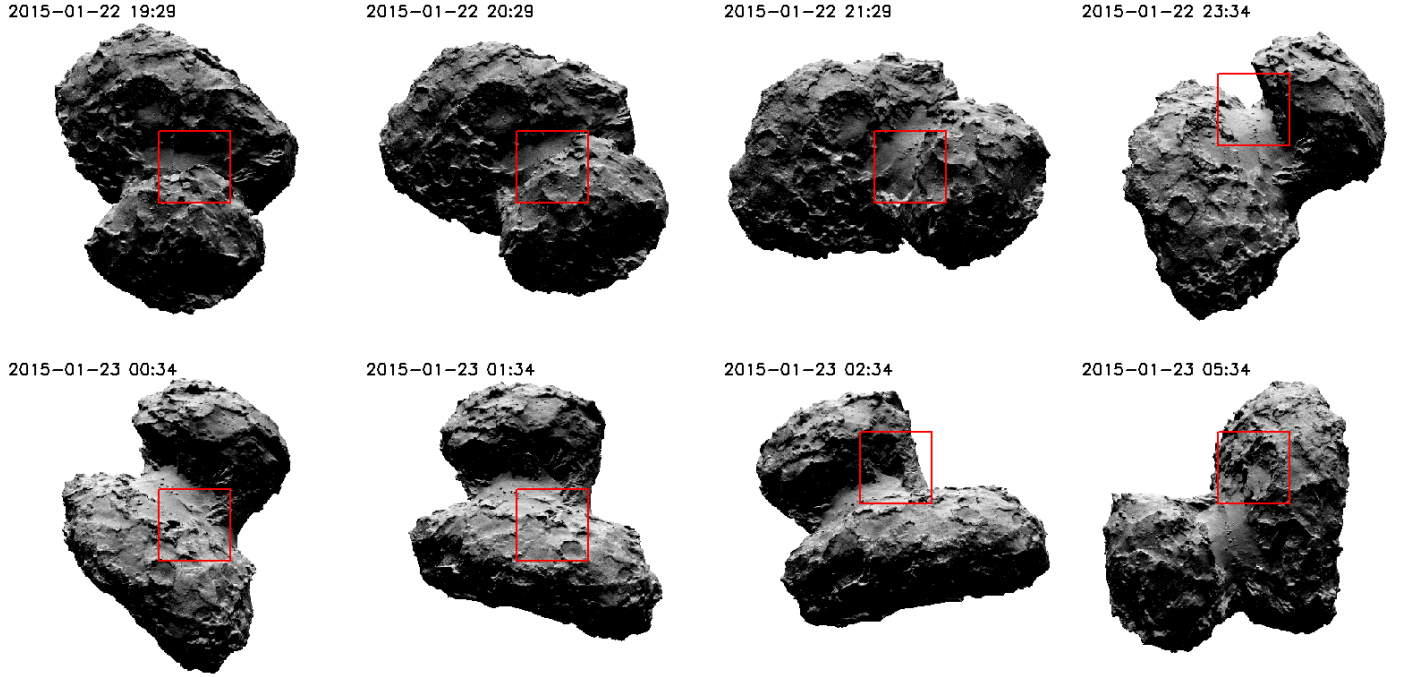
Fig. 7. Orientation of 67P nucleus at the observing time and portion of the nucleus observed for each slope map panel in Fig. 6.
