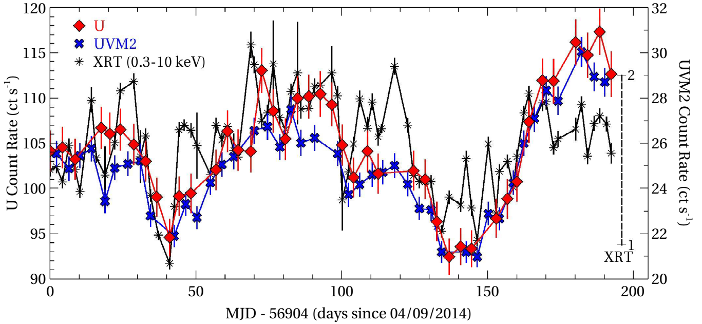
Figure 16. The Swift UVOT light curve of Ark 120 showing the corrected count rates in the U and UVM2 bands. Each point corresponds to a single image / observation. The 0.3–10 keV XRT light curve is overlaid with an additional y-axis scale for comparison.
