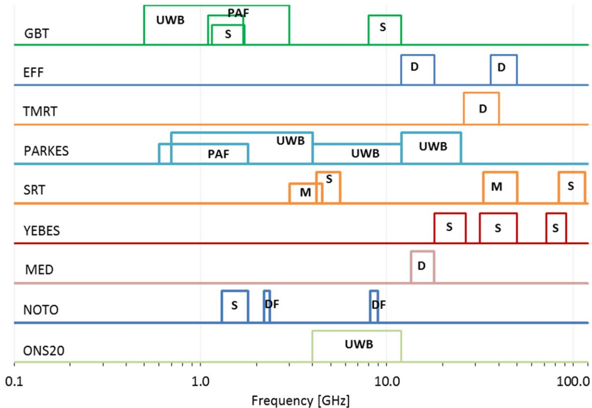
Figure 13. Frequency coverage and category for receivers under development. S = mono-feed; D = dual-feed; M = multi-feed; DF = dual-frequency; PAF = phased array feed; and UWB = UWB-feed.
