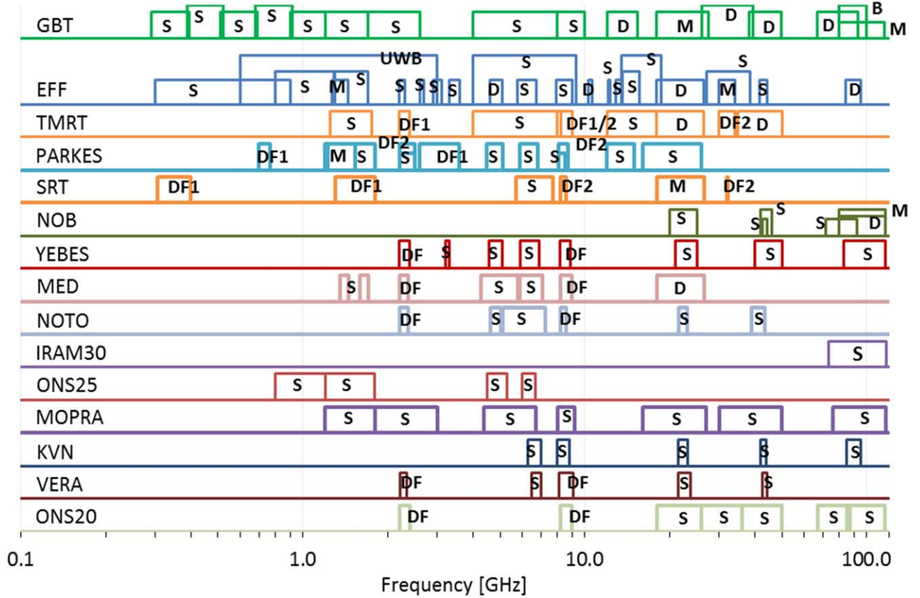
Figure 4. Frequency coverage and category for operational receivers. Receiver categories are: S = mono-feed; D = dual-feed; M = multi-feed; DF = dual-frequency; B = Bolometer; and UWB = UWB-feed. For dual-frequency receivers, the two bands are identified with the same number.
