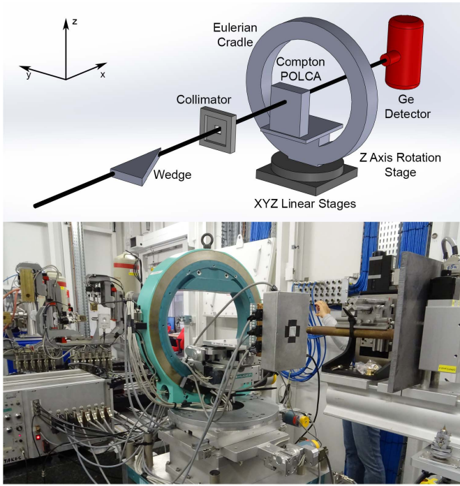
Fig. 2. Top: schematic of the main experimental setup components. Bottom: photograph of the experimental setup inside the ESRF ID15A beamline hut. The rectangular shape box, in front of the Eulerian cradle ring, contains the two-layer Compton-POLCA prototype.
