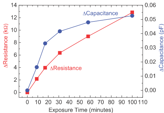
Fig. 3. Dependence of the sensor resistance R (measured at 10 kHz) and capacitance C (at 10 MHz) on the exposure time measured immediately after irradiation with a green LED (peaked at 526 nm wavelength).
