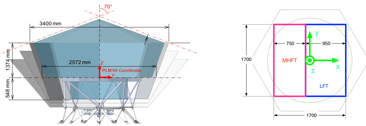
Figure 4. (Left) Usable volume of LFT and MHFT and the PLM coordinate. V-grooves are also shown. The most inner V-groove is at 30 K. The top of the truss is the 5 K structural interface for LFT and MHFT. (Right) Allocated area of LFT and MHFT and the PLM coordinate.
