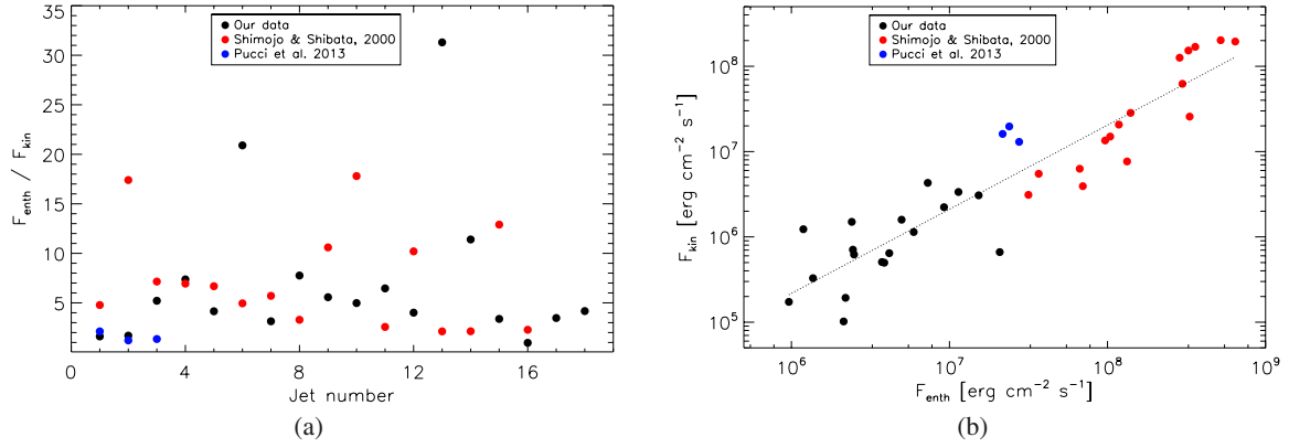
Fig. 7. Left panel a ): ratio between the F_{\text{enth}}/F_{\text{kin}} fluxes ( y -axis), computed for the 18 jets studied here ( x -axis). Right panel b ): enthalpy flux (on the x -axis, logarithmic scale) versus the kinetic flux ( y -axis, logarithmic scale). Data from our analysis are plotted here (black circles), together with those (red and blue circles) from the studies performed by Shimojo & Shibata (2000) and Pucci et al. (2013).
