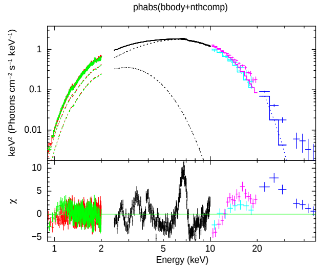
Figure 2. Unfolded E^2 f(E) XMM-Newton /EPIC-pn (black), XMM-Newton /RGS spectra (red and green), INTEGRAL /JEM-X1 and X2 (cyan and magenta), and INTEGRAL /ISGRI (blue). The dashed curves represent the BBODY and the NTHCOMP components (see text). For display purpose only, RGS data have been rebinned with a minimum of 20\sigma and maximum number of energy channels of 20.
