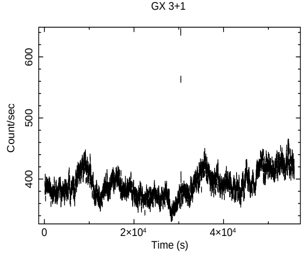
Figure 1. XMM-Newton /EPIC-pn lightcurve in the 0.3–10 keV energy range, corrected for pile-up excising the brightest central column and sampled with bins of 20 seconds. A type-I burst and clear time variability are observed.
