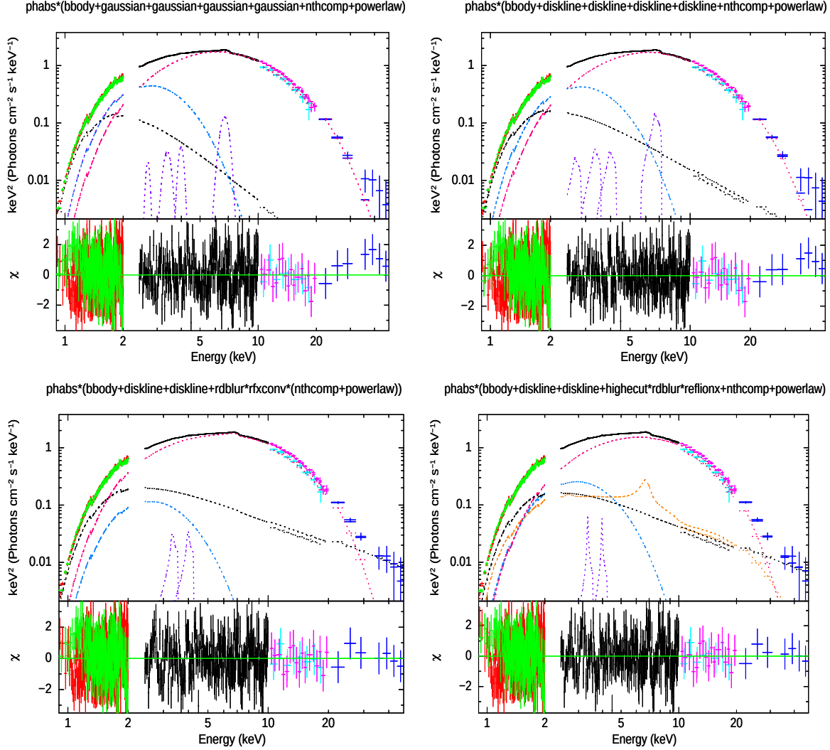
Figure 3. Unfolded E^2 f(E) XMM-Newton/EPIC-pn (black), XMM-Newton/RGS spectra (red, first order, and green, second order), INTEGRAL/JEM-X1 and X2 (cyan and magenta) and INTEGRAL/ISGRI (blue). The top panel shows the best fit with the GAUSSIAN (top-left) or DISKLINE (top-right) models; the bottom panel shows the best fit with the RFXCONV (bottom-left) or REFLIONX (bottom-right) self-consistent models. The dashed curves represent the BBODY (light blue), the NTHCOMP (light red), the POWERLAW (dark grey), the GAUSSIAN or DISKLINE (purple) and the self-consistent (orange) components. For display purpose only, RGS data have been rebinned with a minimum of 20\sigma and maximum number of energy channels of 20.
