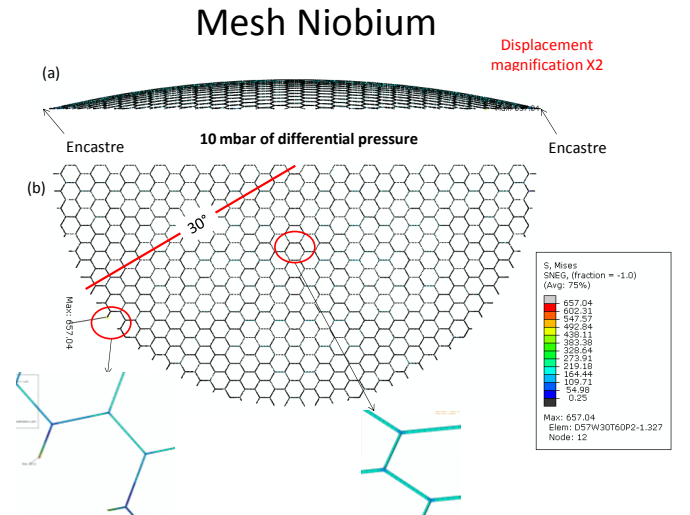
Fig. 5. Von Mises stress distribution over the Nb mesh with magnification of the boundary and center parts; in (a) side view, in (b) top view.
