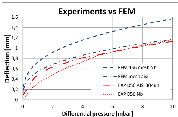
Fig. 7. Comparison between experimental and numerical results for the maximum deflection of both the Nb and steel mesh as a function of the differential pressure.
