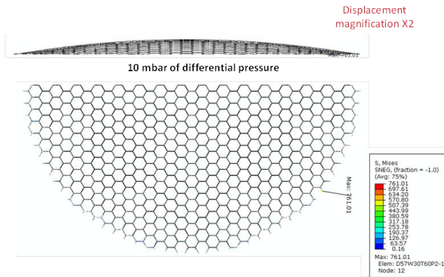
Fig. 6. Von Mises stress distribution over the AISI 304 mesh; in (a) side view, in (b) top view.
