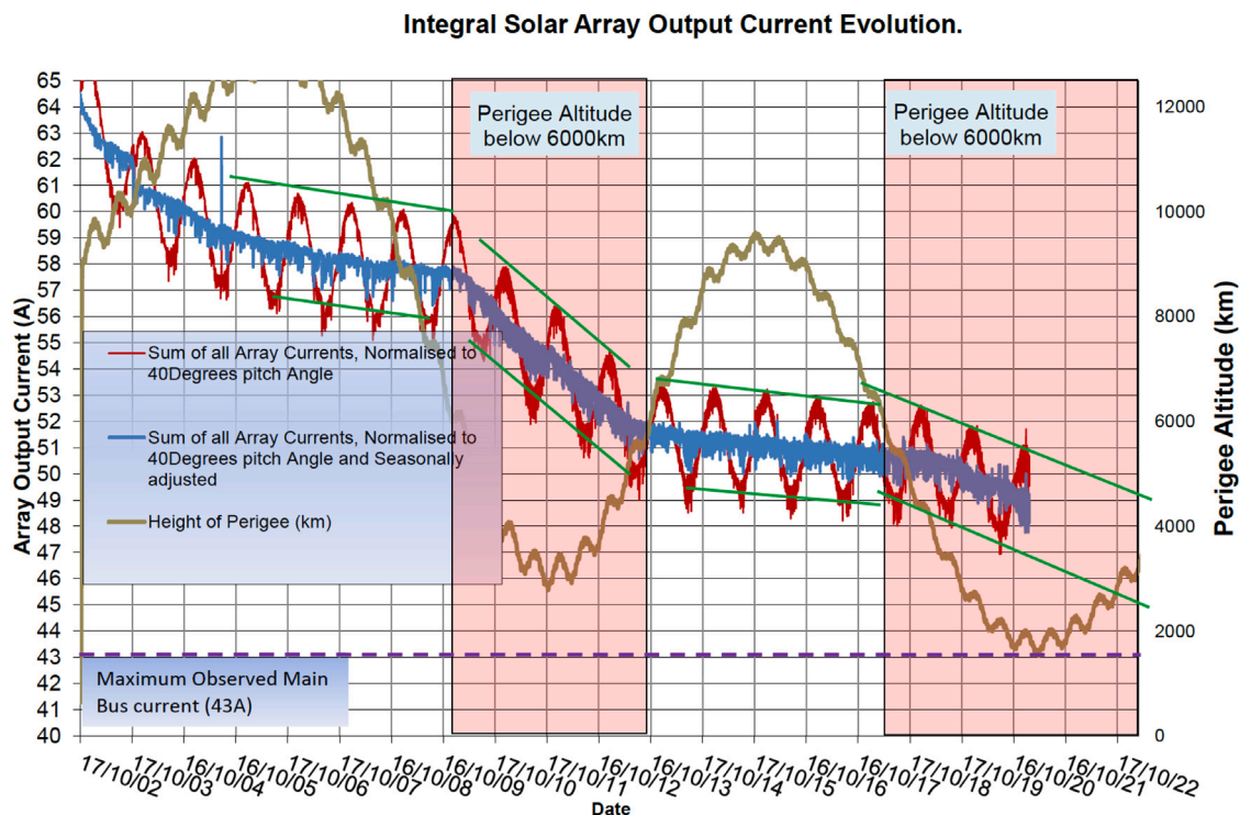
Fig. 15. INTEGRAL worst case Solar array output and perigee altitude evolution.
