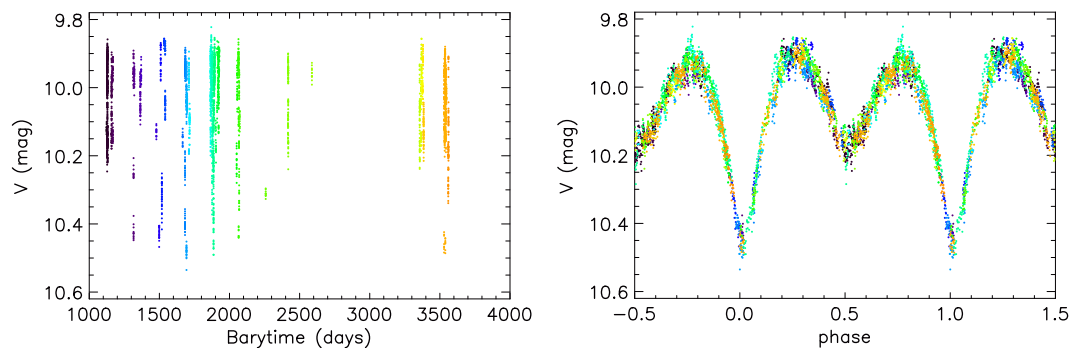
Fig. 10. OMC Optical light curve over 2500 days of the eclipsing binary system IT Nor (IOMC 7864000021). Different colours have been used to distinguish between the different epochs, as shown in the unfolded light curve (left panel). The improvement in the determination of the orbital period of the system ( P_{orb} = 1.75414 \pm 0.00001 days) with respect to previously published data, yielded a perfect phase-folding of the light curve (right panel). This is a representative example of the OMC light curves provided in Alfonso-Garzón et al. (2012) .
