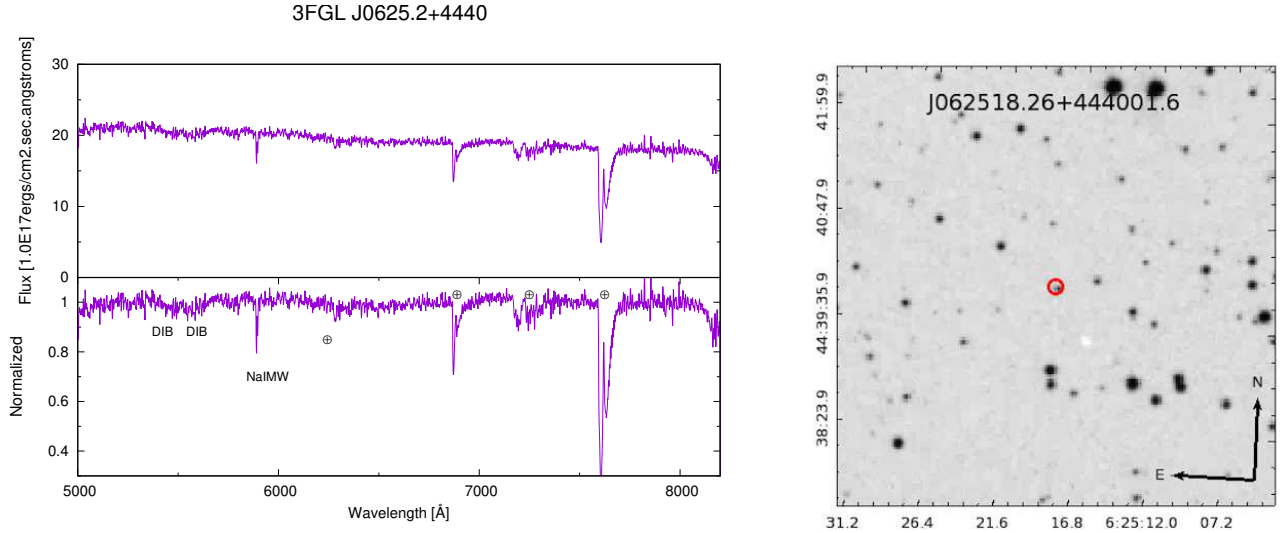
Fig. 12 (Left panel) Top: Optical spectrum of WISE J062518.26+444001.6 associated with 3FGL J0625.2+4440. Bottom: The same spectrum, normalised to highlight features (if any). If present, telluric lines are marked with \oplus , and features due to contamination from diffuse interstellar bands are marked with DIB. If there are any doublets, these are marked with a d. The absorption line at \sim 5890\text{\AA} which is NaI from the Milky Way, is marked as NaIMW. Unidentified lines are marked with a question mark. (Right panel) The finding chart ( 5' \times 5' ) retrieved from the Digitized Sky Survey highlighting the location of the optical source: WISE J062518.26+444001.6 (red circle)
