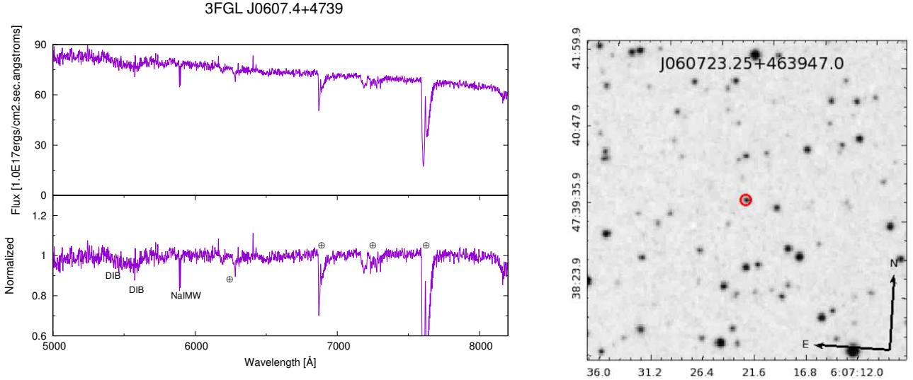
Fig. 10 (Left panel) Top: Optical spectrum of WISE J060723.25+463947.0 associated with 3FGL J0607.4+4739. Bottom: The same spectrum, normalised to highlight features (if any). If present, telluric lines are marked with \oplus , and features due to contamination from diffuse interstellar bands are marked with DIB. If there are any doublets, these are marked with a d. The absorption line at \sim 5890 \text{\AA} which is NaI from the Milky Way, is marked as NaIMW. Unidentified lines are marked with a question mark. (Right panel) The finding chart ( 5' \times 5' ) retrieved from the Digitized Sky Survey highlighting the location of the optical source: WISE J060723.25+463947.0 (red circle)
