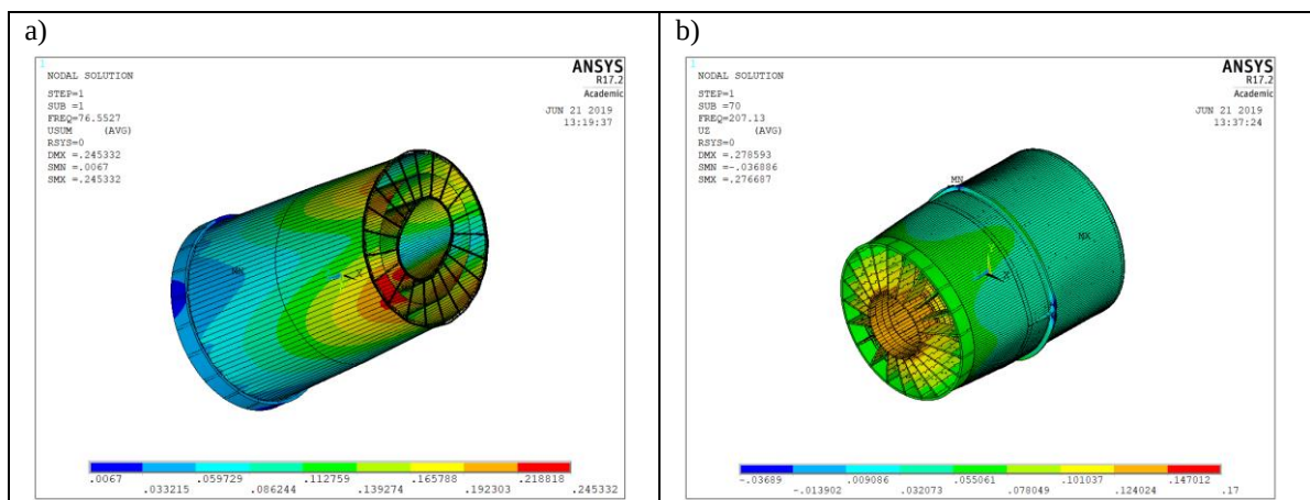
Figure 9—first vibration modes in the lateral direction at the frequency of 76.5 Hz (the external case is not shown for clarity) (a) and in the axial direction (207 Hz) (b). Both figures refer to the hard-mounting case.
