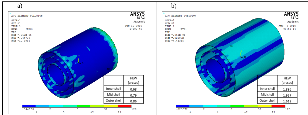
Figure 7 – Optical mirror shells maps: contribution on the angular resolution (HEW, arcsec) due to thermal load ( \Delta T=1^\circ\text{C} , uniform) with the \Phi_{\text{min}} mask (a) and without the \Phi_{\text{min}} mask (b) in the case of hard-mounting.
