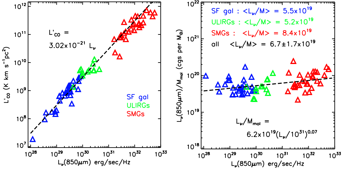
Figure A1. Left: The CO(1-0) luminosity and L_\nu at 850\mu\text{m} are shown for three samples of galaxies – normal low- z star forming galaxies, low- z ULIRGs and z \sim 2 SMGs. All galaxies were selected to have global measurements of CO (1-0) and Rayleigh-Jeans dust continuum fluxes. The large range in apparent luminosities is enhanced by including the high redshift SMGs, many of which in this sample are strongly lensed. Right: The ratio of L_\nu at 850\mu\text{m} to M_{\text{ISM}} is shown for the three samples of galaxies, indicating a very similar proportionality constant between the dust continuum flux and the molecular masses derived from CO(1-0) emission. The molecular masses were estimated from the CO (1-0) luminosities using a single standard Galactic X_{\text{CO}} = 3 \times 10^{20} \text{ N(H}_2\text{) cm}^{-2} (\text{K km s}^{-1})^{-1} .
