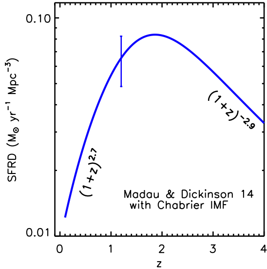
Figure 15. The evolution of the cosmic star formation rate density (SFRD) from Madau & Dickinson (2014) is shown for comparison with the overall evolution of ISM content in Figure 14-Left. A typical uncertainty is shown as 0.1 dex (see Madau & Dickinson 2014) (The relative scaling of z and the SFRD is the same as that in Figure 14.)
