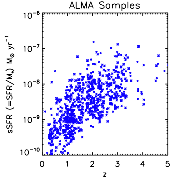
Figure 3. The distributions of sSFR and redshifts for the objects which were detected are shown.
