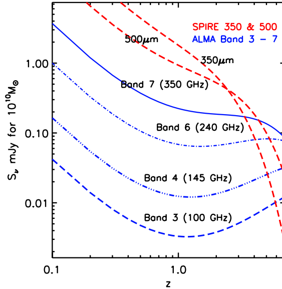
Figure A2. The expected continuum fluxes for the ALMA bands at 100, 145, 240 and 350 GHz and for SPIRE 350 and 500\mu\text{m} for M_{\text{ISM}} = 10^{10} M_\odot derived using the empirical calibration \alpha = 6.7 \times 10^{19} (Scoville et al. 2016), an emissivity power law index \beta = 1.8 and including the RJ departure coefficient \Gamma_{\text{RJ}}(25\text{K}) . Since the point source flux sensitivities of ALMA in the 4 bands are quite similar, the optimum strategy is to use Band 7 out to z \sim 2-3 ; above z = 3 . Lower frequency ALMA bands are required to avoid large uncertainties in the RJ correction.
