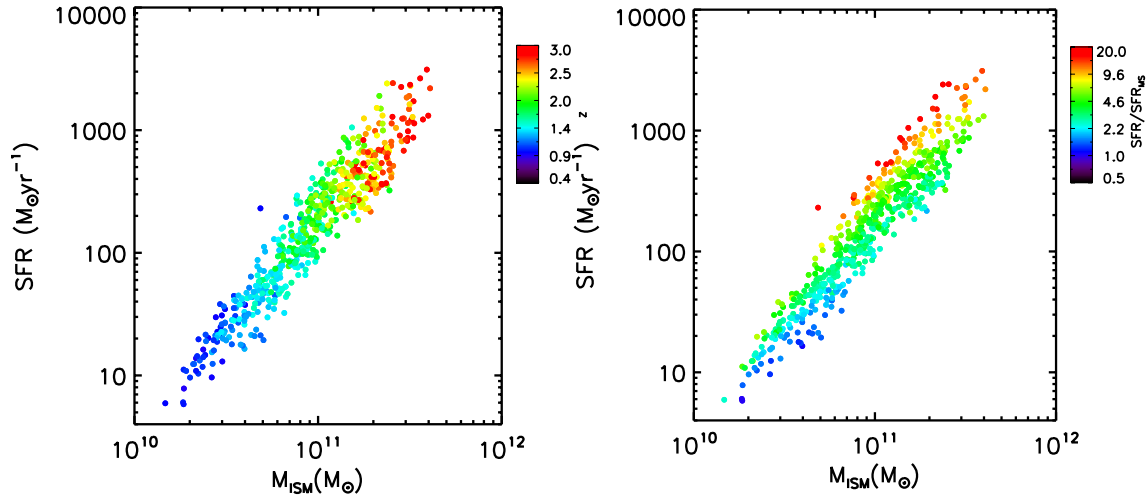
Figure 8. The fitted ISM masses and observed SFRs are shown with color coding based on redshift and s\text{SFR} relative to the MS. The dominant dependence of the SFR is on M_{ISM} , with relatively weaker dependencies on z and the MS-Ratio.
