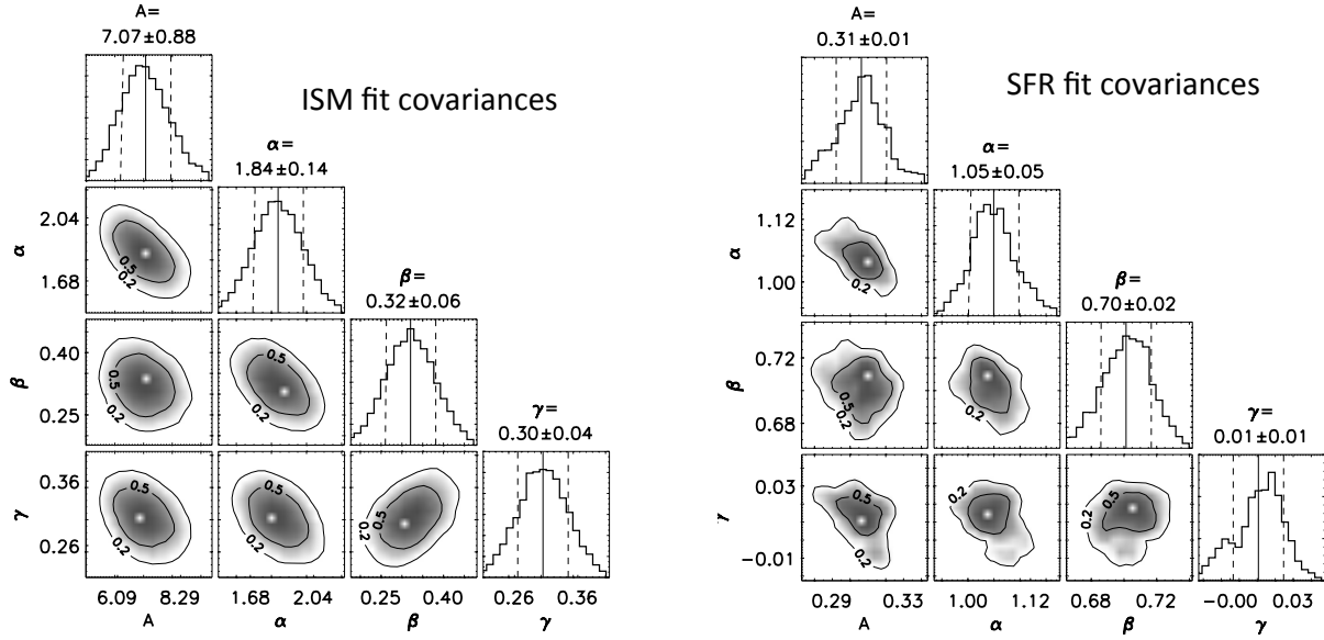
Figure C1. The covariance distributions for the fits obtained in Equations 6 and 7 are shown in the Left and Right panels, respectively. The parameters A , \alpha , \beta and \gamma correspond to the lead scale factor and the exponents in the Equations.
