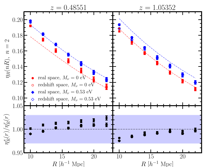
Figure 3. The clustering ratio smoothed on the scale R and at correlation length r = nR, n = 2 as a function of the smoothing scale. We show in red the measurements in the \Lambda\text{CDM} simulation and in blue the ones in the simulation with the highest neutrino mass, M_\nu = 0.53 \text{ eV} , which represent the two extreme cases for the neutrino mass considered in this work. Filled dots are measurements in real space, while empty dots represent redshift space measurements. In the bottom panel the ratio between the clustering ratio in redshift space over the real space case is shown. Since on linear scales the monopole contribution coming from redshift-space distortions enhances the correlation function and the variance by the same multiplicative factor, we expect the clustering ratio to be unaffected. The ratio between redshift and real space measurements is, in fact, of order 1 with an accuracy better than 3 per cent. This trend is confirmed from measurements at redshift z = 1.05352 (right), being the matter growth more linear at higher redshifts.
