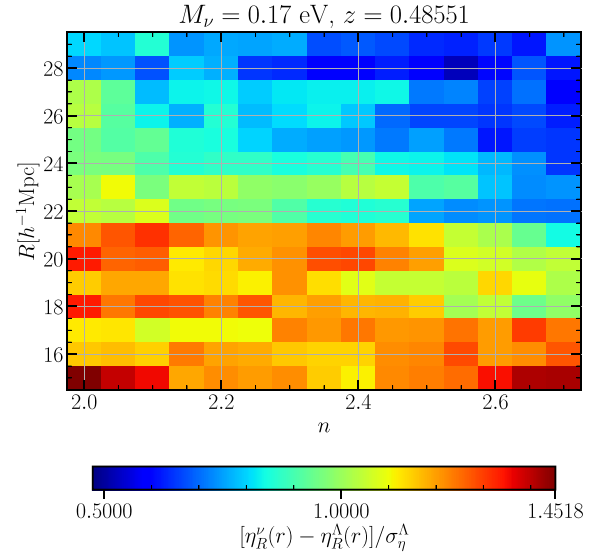
Figure 4. The effect of neutrinos on the clustering ratio compared to a \Lambda CDM cosmology. In the (n, R) plane, we plot colour contours corresponding to (\eta_R(r, v) - \eta_R(r, \Lambda\text{CDM})/\sigma_\eta(\Lambda\text{CDM})) . As expected, the sensitivity to the neutrino total mass increases at small smoothing scales and correlation lengths (red regions).
