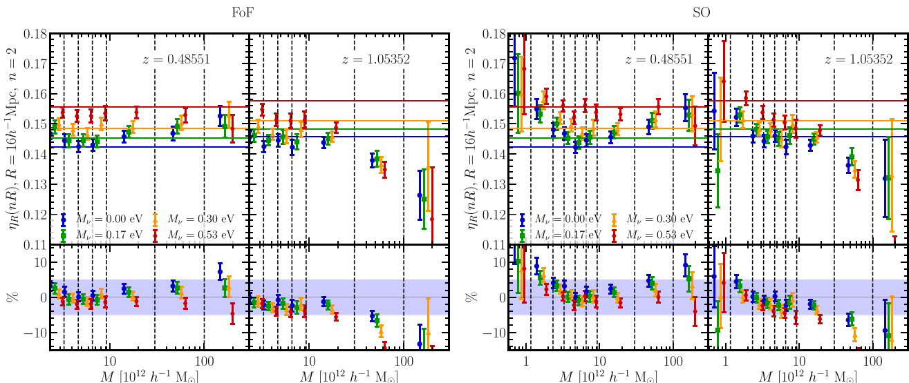
Figure 2. Dependence of the clustering ratio on the mass of haloes identified via FoF (left-hand panel) and spherical overdensity (SO, right-hand panel) at redshift z = 0.48551 and z = 1.05352 for all the neutrino masses. The smoothing radius is R = 16 h^{-1} \text{ Mpc} and the correlation length is twice the smoothing radius. Symbols with error bars show measurements in the simulations, while solid lines represent the theoretical expectation for the cold matter. In the bottom panel we show the relative difference between the measurements and theoretical predictions, the shaded area represents a -5, +5 per cent deviation.
