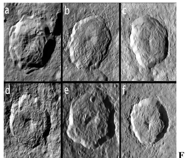
fig. 26. Comparison of immature complex craters on Ceres (a–c) and on icy Saturnian satellites (d–f). Ceres craters are between 20 and 40 km across. Crater (d) is Telemachus ( D = 95 km) and (f) is Sagaris ( D = 45 km), also highlighted in Fig. 10. Craters shown at similar apparent diameter (and at different scales) to facilitate structural comparison.
