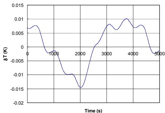
Figure 9-5. Expected temperature oscillation at the 30 GHz front-end radiometers considering a Sorption
