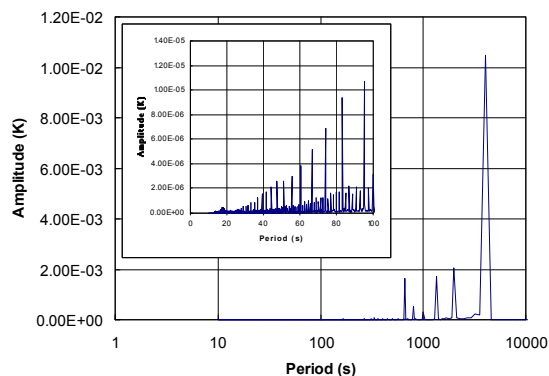
Figure 9-5. Expected temperature oscillation at the 30 GHz front-end radiometers considering a Sorption
