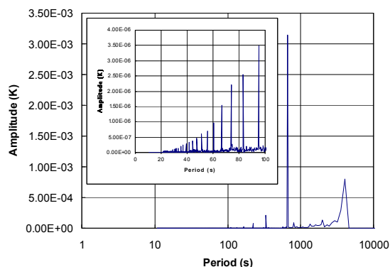
Figure 9-3. Same as in Figure 9-1 for the 70 GHz front-end radiometers.
