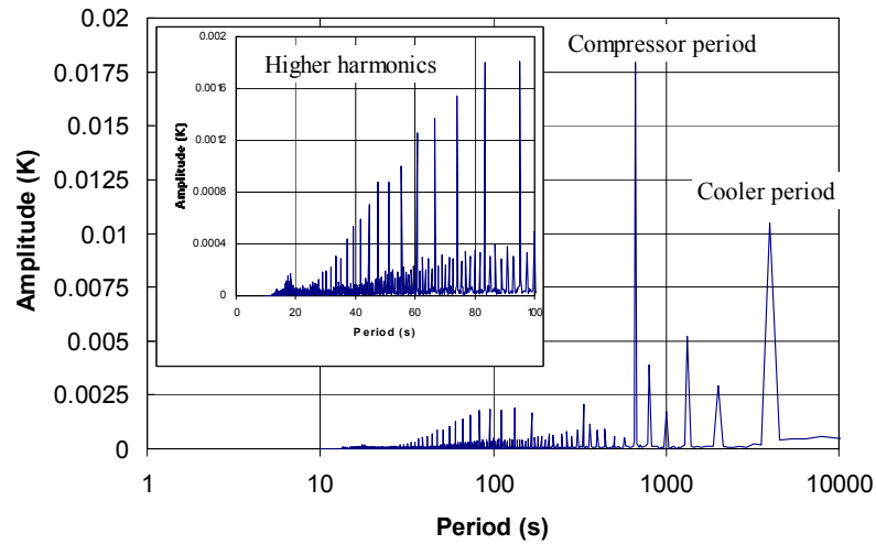
Figure 3-5. Fourier transform (amplitude vs. period) of the temperature oscillation in Figure 3-4. The figure shows that the presence of a non-homogeneous compressor bed determines an increase in the 4000s component (at the level of about 20 mK peak-to-peak) and of the high frequency tail, with the main spin-synchronous components (60s and 30s period) at the level of about 2.5 mK peak-to-peak and 0.4 mK peak-to-peak, respectively.
