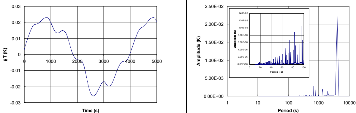
Figure 9-10. Same as in Figure 9-9 for the 44 GHz front-end radiometers.
