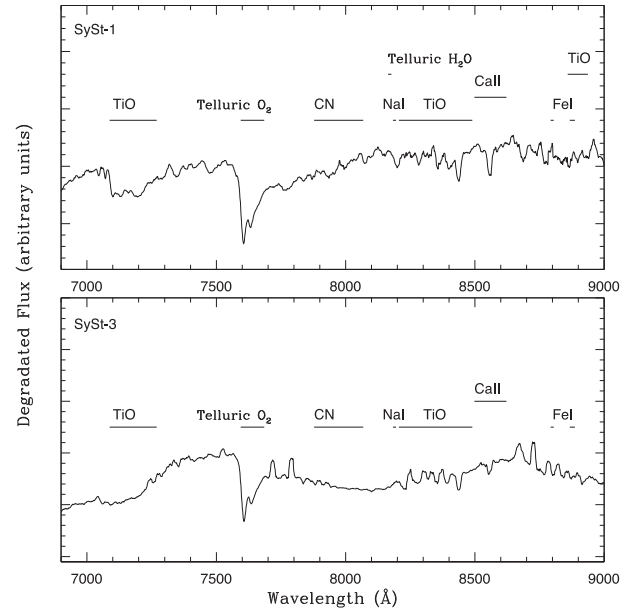
Figure 3. The 6900 – 9000 \text{ \AA} range of the red spectrum of NGC 205 SySt-1 and 3, smoothed to match the spectral resolution of the Kirkpatrick, Henry & McCarthy (1991) catalogue ( 18 \text{ \AA pixel}^{-1} ). Following Kirkpatrick et al. (1991), the most prominent features, key to determine the spectral type, are identified. (i) The CN bands are obvious in supergiants, weaker in giants and not seen in dwarfs. (ii) The TiO whose head band is at 8206 \text{ \AA} is very strong in mid-M. (iii) The Ca II bands are strong from late-K to mid-M, strongest in supergiants and very weak in dwarfs. (iv) Fe I absorptions (at 8793 – 8805 \text{ \AA} ) are found in giants as well as supergiants.
