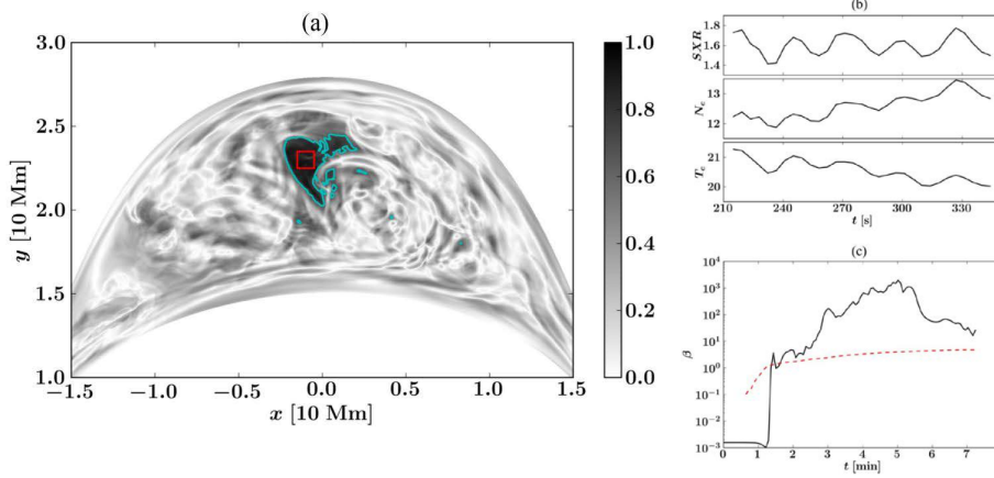
Fig. 3 (a) Correlation coefficient between the oscillatory signals within the turbulent region. The cyan contour label the value at 0.7. (b) Temporal evolution of SXR flux, average density, and temperature within the red box in panel (a). (c) Temporal evolution of average plasma beta in the red box (black solid line). Adapted from Ruan et al. (2019) with permission.
