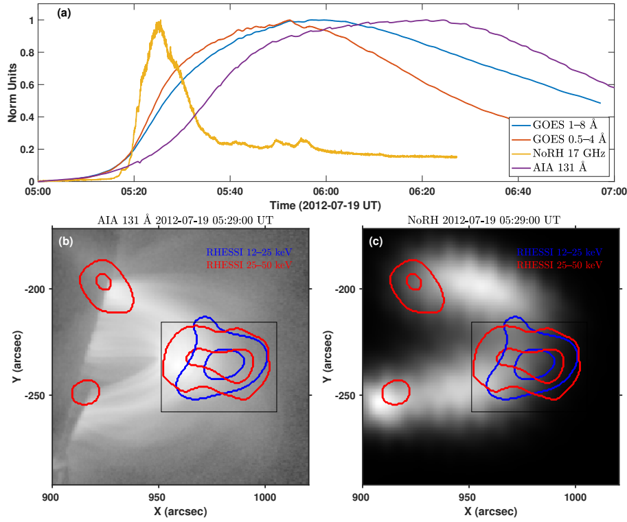
Fig. 5 (a) light curves showing the rise and decay of a solar flare recorded by GOES, NoRH and AIA 131 Å (b) Coronal loop system observed by AIA 131 Å channel. (c) NoRH synthetic image of 17 GHz. The blue and red contours label the emission levels of RHESSI 12-25 keV and 25-50 keV X-ray emissions. Adapted from Yuan et al. (2019) with permission.
