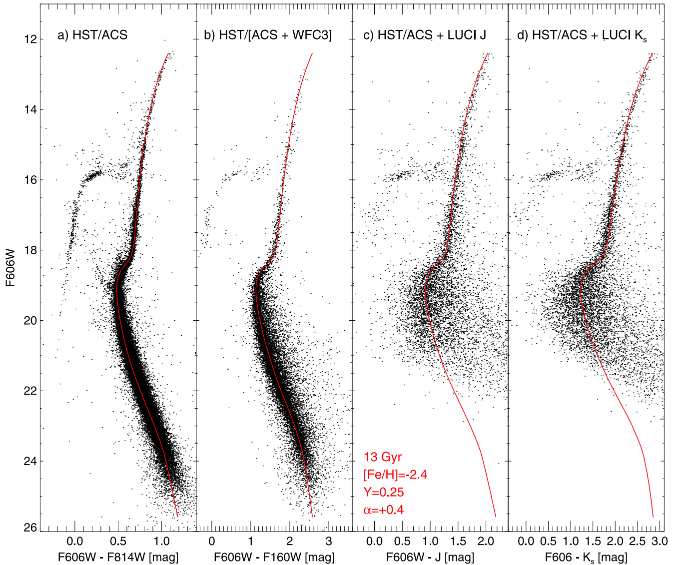
Figure 6. Optical and NIR CMDs based on HST data superimposed with the same isochrone for the labeled parameters.
