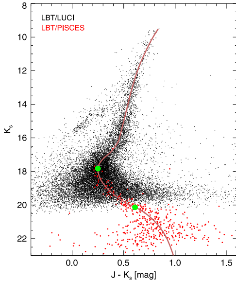
Figure 8. ( K, J - K ) CMDs from LBT data (black: LUCI; red: PISCES) superimposed with the derived ridge line. The big dots mark the MSTO and MSK points.
