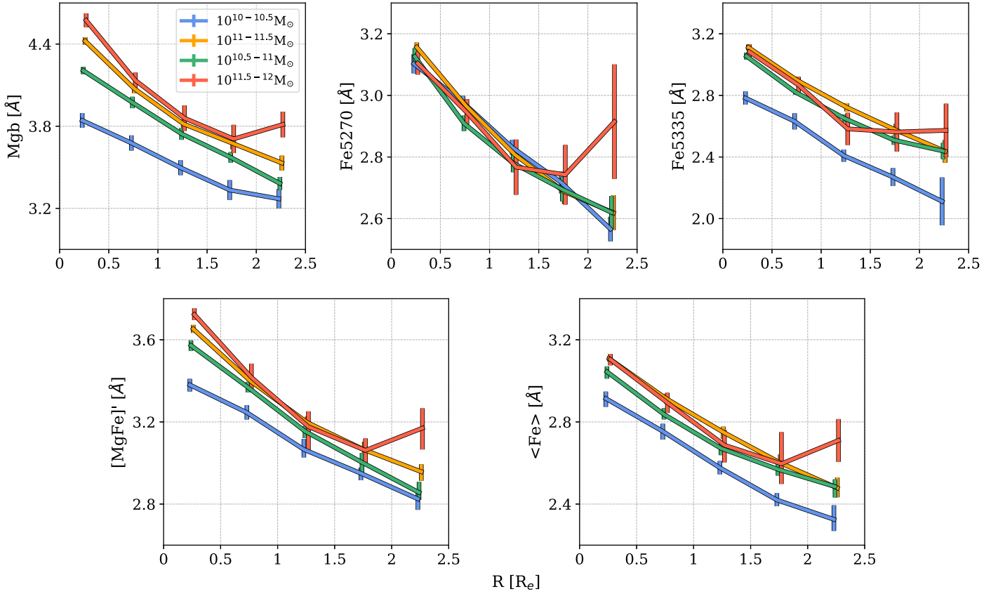
Figure 6. Median radial profiles of Mgb, Fe5270, Fe5335, [MgFe]', and \langle \text{Fe} \rangle for MaNGA ETGs as a function of M_* . These profiles are based on measurements made by the MaNGA DAP. The profiles flatten at the highest M_* , in consistency with Figure 2.
