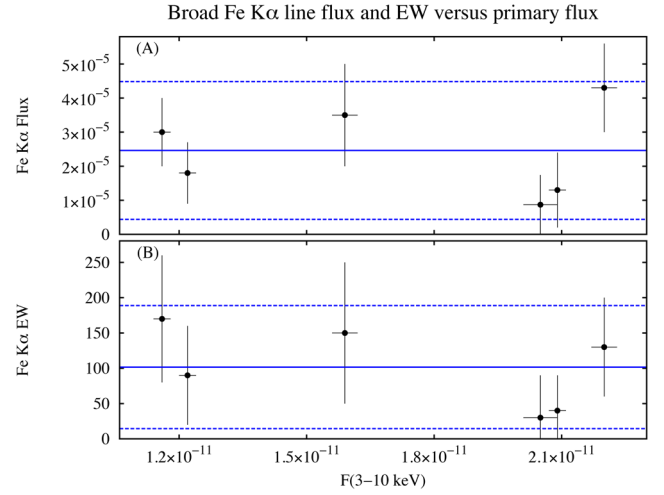
Figure 5. Parameters of the broad Fe K \alpha line at 6.4 keV, plotted against the primary flux in the 3–10 keV band. Panel (A): the line flux in units of photons cm -2 s -1 . Panel (B): the line equivalent width (EW) in units of eV. Error bars denote the 1 \sigma uncertainty. The blue solid lines represent the mean value for each parameter, while the blue dashed lines represent the standard deviation.
