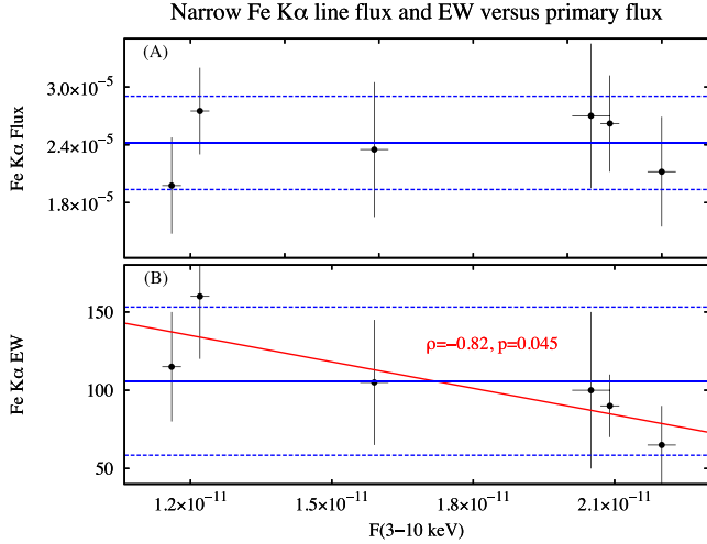
Figure 4. Parameters of the narrow Fe K \alpha line at 6.4 keV, plotted against the primary flux in the 3–10 keV band. Panel (A): the line flux in units of photons cm -2 s -1 . Panel (B): the line equivalent width (EW) in units of eV. Error bars denote the 1 \sigma uncertainty. The blue solid lines represent the mean value for each parameter, while the blue dashed lines represent the standard deviation (i.e. the root mean square of the deviations from the mean). The red line represents a linear fit to the data.
