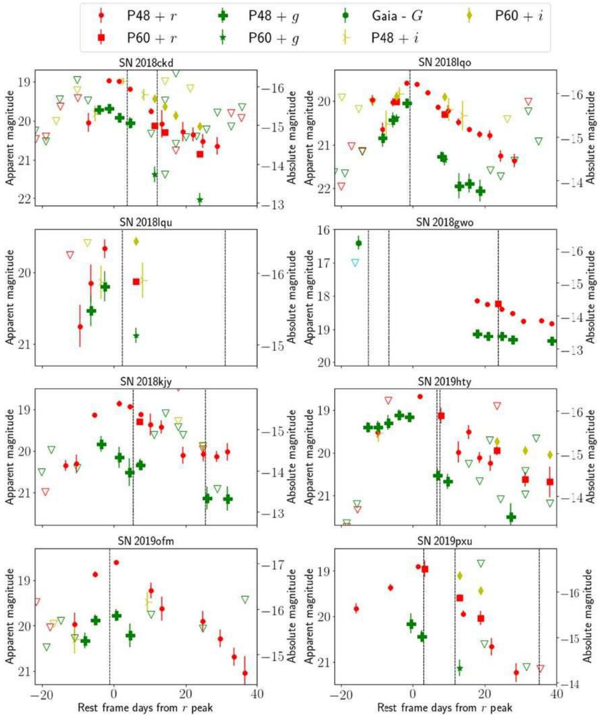
Figure 3. Photometric evolution near peak light of the Ca-rich gap transients presented in this sample, with time presented with respect to the r -band light curve of the individual sources (corrected for Galactic extinction). Filled symbols denote detections from forced photometry on the ZTF difference images (see figure legend), while hollow inverted triangles denote 5\sigma upper limits at the position of the transient. Red points denote r -band photometry, green points denote g -band photometry, yellow points denote i -band photometry, and cyan points denote photometry in the clear filter. The vertical dashed lines denote the epochs of spectroscopy. For SN 2018gwo, we also show public TNS photometry from Gaia & Wiggins (2018) (see legend).
