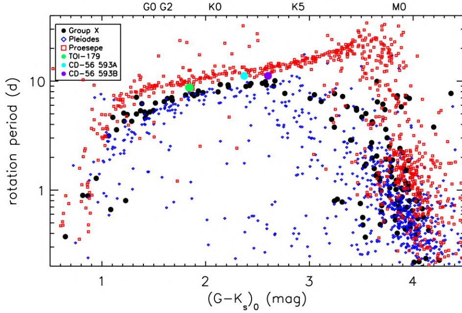
Fig. A.5: Rotation period of TOI-179 and CD-56 593A and B vs. (G-K)_0 color (green, cyan, and purple filled circles, respectively), compared to the members of the Pleiades and Praesepe open clusters (Rebull et al. 2016, 2017, plotted as blue diamonds and red squares, respectively) and Group X moving group (Messina et al. 2022, plotted as black circles). Only one photometric period is measured for CD-56 593, spatially unresolved in TESS images, and we are unable to determine to which component it belongs. The data are plotted in the figure for the colors of both components.
