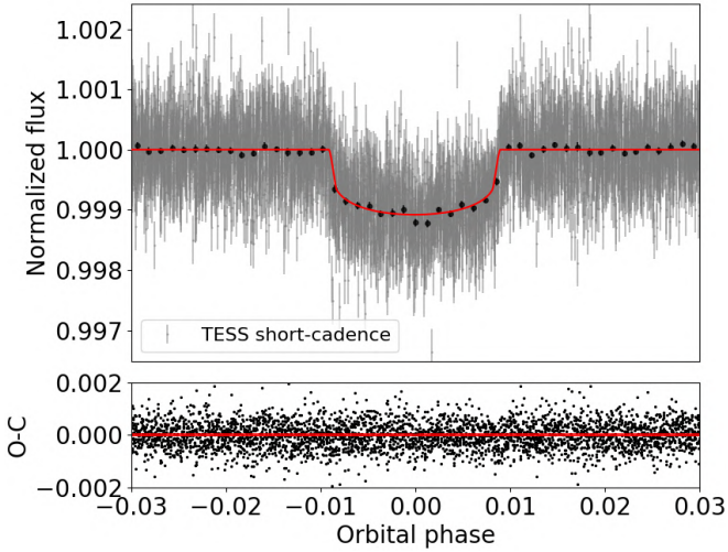
Fig. 8. Best-fit transit signal of TOI-179 b based on TESS short-cadence photometry (Table 3). Model residuals O-C are shown in the bottom panel.
