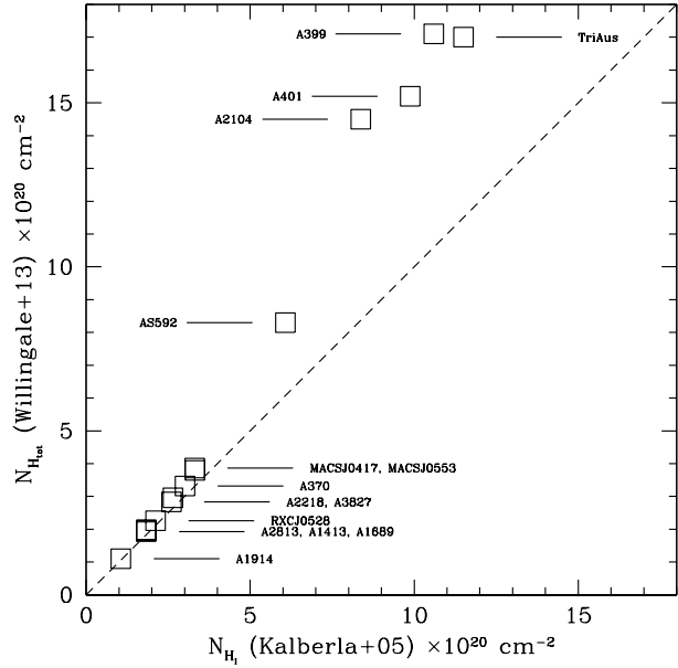
Figure 1. Comparison between the H_I density column from Kalberla et al. (2005) and the total ( H_I + H_2 ) density column from Willingale et al. (2013). The dashed line indicates the linear correlation as a reference.
