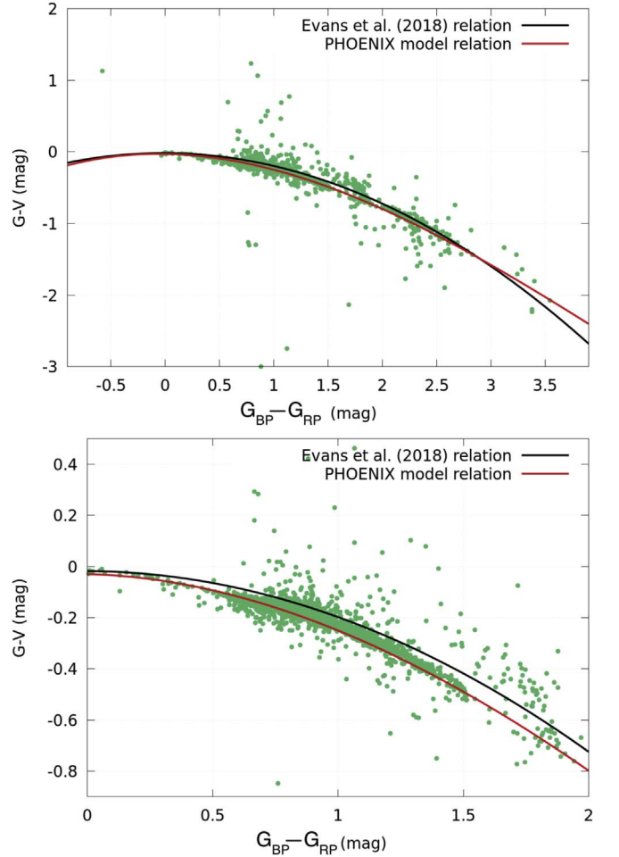
Figure 4. The top panel presents a comparison of our synthetic G - V colors as a function of G_{BP} - G_{RP} (polynomial red line fit) with a similar relation by Evans et al. (2018) shown in black. The bottom panel shows a close-up of the solar-color region. The points represent actual measurements for a set of stars from TICv7.
