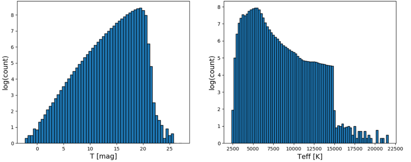
Figure 14. TICv8 distributions of T (left) and T_{\text{eff}} (right).
