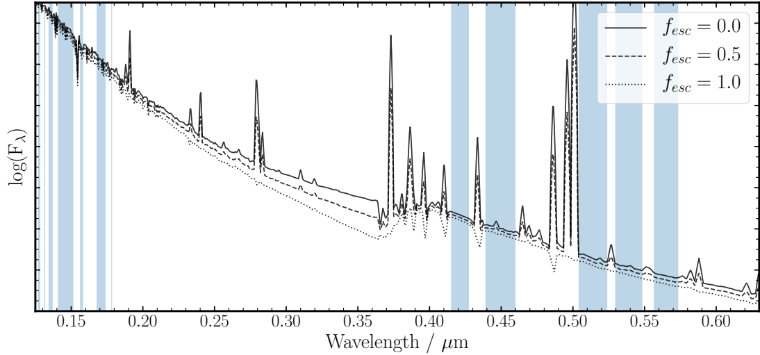
Figure 5. The intrinsic FiBY-BPASSv2-300bin SED across the wavelength region 0.125\mu\text{m} < \lambda < 0.63\mu\text{m} assuming different values for the escape fraction of ionizing photons ( f_{esc} ). It can be seen that some wavelength regions are extremely sensitive to the nebular spectrum and therefore unsuitable to use when fitting the attenuation curve (see text for details). The blue shaded areas show the wavelength regions we defined as suitable to use. These wavelength pixels satisfied the following criteria: (i) a maximum nebular contribution of 10%; (ii) free from any strong stellar absorption/emission features.
