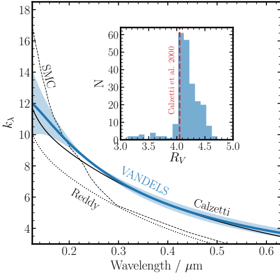
Figure 10. The total-to-selective attenuation curve k_\lambda for our fiducial intrinsic SED template (FiBY-BPASSv2-300bin). Individual k_\lambda curves were derived using Equation 6 for each of the 229 galaxies which had an attenuation curve solution. The blue line shows the average across all individual galaxies, with the shaded region showing the \pm 1\sigma scatter. A selection of k_\lambda curves from the literature are also shown and labeled. The inset panel shows the distribution of R_V values for all 229 galaxies obtained using Equation 5. The average across all galaxies is R_V = 4.18 \pm 0.29 , which is in good agreement with the original determination for a Calzetti law of R_V = 4.05 \pm 0.80 (Calzetti et al. 2000, indicated by the dashed orange line).
