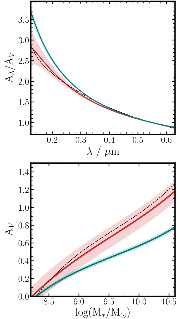
Figure 7. Testing the accuracy of our attenuation curve fitting method with simulations. The top panel shows the average attenuation curve shape ( A_\lambda/A_V ) recovered from a simulation of 1000 SEDs which have been reddened with a Calzetti law, drawing A_V values from the McLure et al. (2017a) A_V - M_* relation. The blue line shows the A_\lambda/A_V relation recovered using the full 0.12 - 0.63\mu\text{m} wavelength range in the fitting, while the red line shows the A_\lambda/A_V recovered using only the restricted wavelength regions given in Table 2. The black dashed line shows the input A_\lambda/A_V relation. The bottom panel shows the recovered A_V - M_* relation for both these scenarios, again compared to the input relation (black dashed line). In both panels, shaded regions show the \pm 1\sigma error on the recovered relations.
