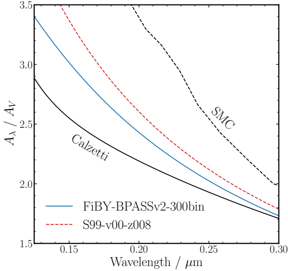
Figure 11. The average attenuation curve shape ( A_\lambda/A_V ) for galaxies with \log(M_*/M_\odot) < 9.0 . The solid blue line shows our fiducial FiBY-BPASSv2-300bin template and the dashed red line shows the S99-v00-z008 template. For comparison we show the Calzetti law (solid black line) and the SMC extinction law (dashed black line). It can be seen that we find some tentative evidence for a steepening of the attenuation curve at the lowest masses, though still no evidence for an attenuation law as steep as the SMC extinction curve.
