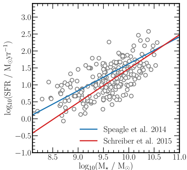
Figure 1. The position of our VANDELS sample in the M_{\star} -SFR plane. Masses and star-formation rates were derived using the SED fitting code LEPAHRE (see text for details). For comparison, the blue and red lines show two independent determinations of the main sequence of star formation at z = 3.5 from Speagle et al. (2014) and Schreiber et al. (2015) respectively. It can be seen that the galaxies in our sample are consistent with being typical star-forming galaxies at z = 3.5 .
