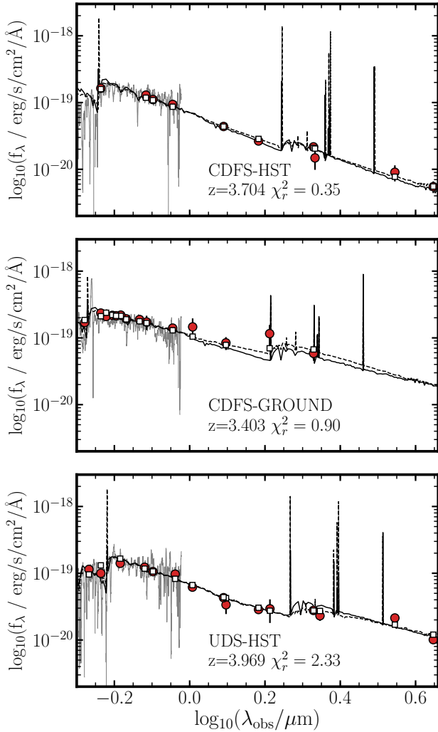
Figure 2. The UV-to-optical spectral energy distributions for three galaxies in our sample. In each panel, the red circular data points show the observed photometry while black solid/dashed spectra show the best-fitting LePhare/EAZY templates respectively. The open squares show the synthetic photometry of the best-fitting EAZY template through the observed filters. The grey spectra at \lambda \approx 0.5 - 1.0 \mu\text{m} ( \log(\lambda/\mu\text{m}) \approx -0.3 - 0.0 ) are overlays of the observed VANDELS spectra, which we used to accurately determine the redshift of the galaxies.
