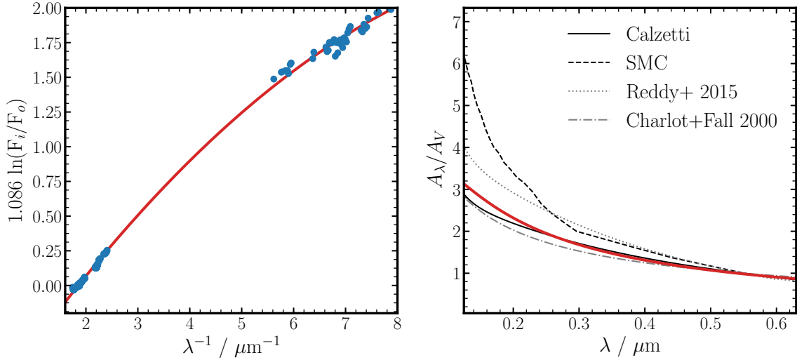
Figure 6. The left-hand panel shows an attenuation curve fit for one galaxy in our sample as described in Section 3, with the wavelength pixels used for the fitting shown as the blue dots (see text for discussion). The final best-fitting solution is shown by the solid red curve. The resulting fit, translated into A_\lambda/A_V versus \lambda is shown in the right-hand panel and is compared to the corresponding curves for the Calzetti et al. (2000), Reddy et al. (2015) and Charlot & Fall (2000) attenuation curves, and the SMC extinction curve of Gordon et al. (2003). For this particular galaxy the solution suggests a grey, Calzetti-like, shape.
