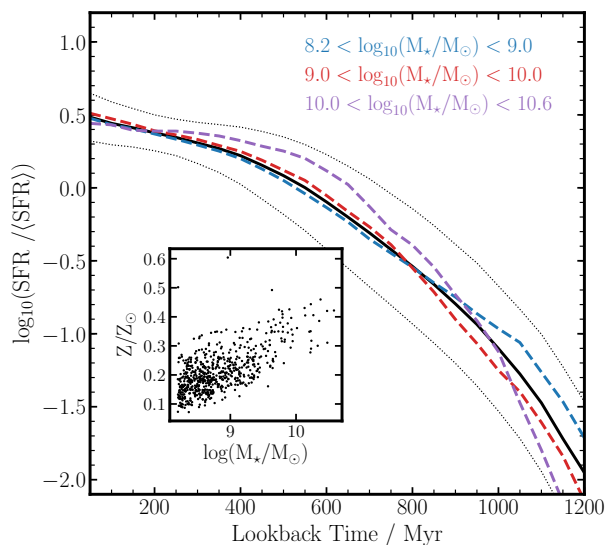
Figure 3. The average normalised star-formation histories and metallicities of 628 simulated galaxies extracted from the FiBY simulation at z = 4 , covering the stellar mass range 8.2 \leq \log(M_*/M_\odot) \leq 10.6 . The black solid curve shows the mean normalised star-formation history with the black dotted curve representing the \pm 1\sigma scatter. The vast majority of the galaxies have self-similar, rising, star-formation histories with an average UV-weighted metallicity of \langle Z/Z_\odot \rangle = 0.21 \pm 0.07 (inset panel). The consistency of star-formation histories is further illustrated by the three colored dashed curves, which show the mean star-formation history in three stellar mass bins, with the corresponding stellar mass ranges given in the upper right-hand corner. As discussed in the text, this conformity of star-formation history results in the intrinsic UV to optical SED shape of all galaxies being consistent to within \approx 10\% (averaged across all wavelengths). This is the basis of our assumption that the observed SED shapes can be compared to a single common intrinsic SED shape, allowing us to directly probe the attenuation curve.
