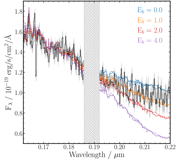
Figure 12. Investigating evidence for excess attenuation at 2175Å from a composite of 122 VANDS spectra at 3.0 \leq z \leq 3.5 ( \langle z \rangle = 3.288 ). The grey spectrum is the composite VANDS spectrum with the grey shaded region representing the \pm 1\sigma error. The hatched region around \lambda \sim 0.19\mu\text{m} masks the \text{C III]}\lambda 1909 emission line. The solid and dashed coloured curves show, respectively, the FiBY-BPASSv2-300bin and S99-v00-z008 templates reddened using the Noll et al. (2009) attenuation curve assuming four values of the 2175Å bump strength ( E_b ; see text for details). For each value of E_b the templates have been attenuated with A_V = 0.8 assuming the Calzetti A_V - M_* relation at the median mass of the galaxies contributing to the stack ( \log(M_*/M_\odot) = 9.71 ; see Fig. 9).
