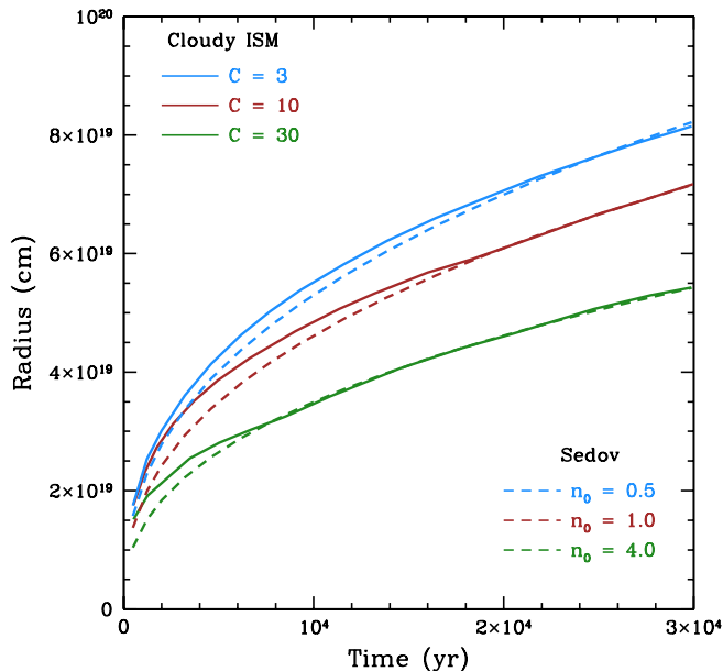
FIG. 9.— SNR radius evolution for expansion in a cloudy ISM (solid), and the Sedov solution (dashed) for evolution into a uniform medium, both for E_{51} = 1 . The cloudy ISM curves (from Slavin et al. 2017) assume density values of 0.25(25) \text{ cm}^{-3} for the intercloud (cloud) regions. The value of C corresponds to the ratio of the cloud mass to that of the intercloud medium. The Sedov solution curves provide reasonable approximations assuming densities roughly connected to the evaporated cloud density in the cloudy ISM model.
