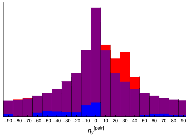
Figure 2. Normalized distribution of \eta_{\gamma}^{[pair]} for all pairs of photons (from the same GRB) within our data set. For bins where the observed population is higher than expected we color the bar in purple up to the level expected, showing then the excess in red. For bins where the observed population is lower than expected the bar height gives the expected population, while the blue portion of the bar quantifies the amount by which the observed population is lower than expected.
