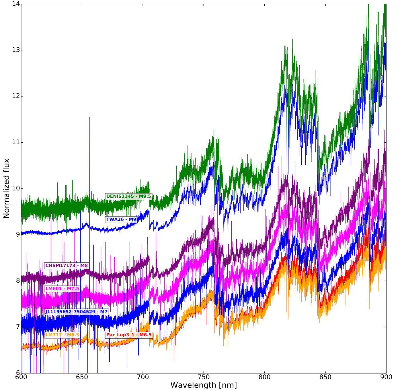
Fig. C.3. Spectra of Class III YSOs with spectral type later than M6 ordered according to their spectral type and normalized at 750 nm.
