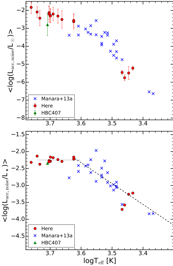
Fig. 8. Luminosity of chromospheric emission lines converted into L_{\text{acc, noise}} as a function of the logarithm of the effective temperature obtained from the spectral type for all the Class III targets discussed here. In the bottom plot the values of L_{\text{acc, noise}} are normalized by the stellar luminosity, and the lines represent the fit reported in Eq. (1).
