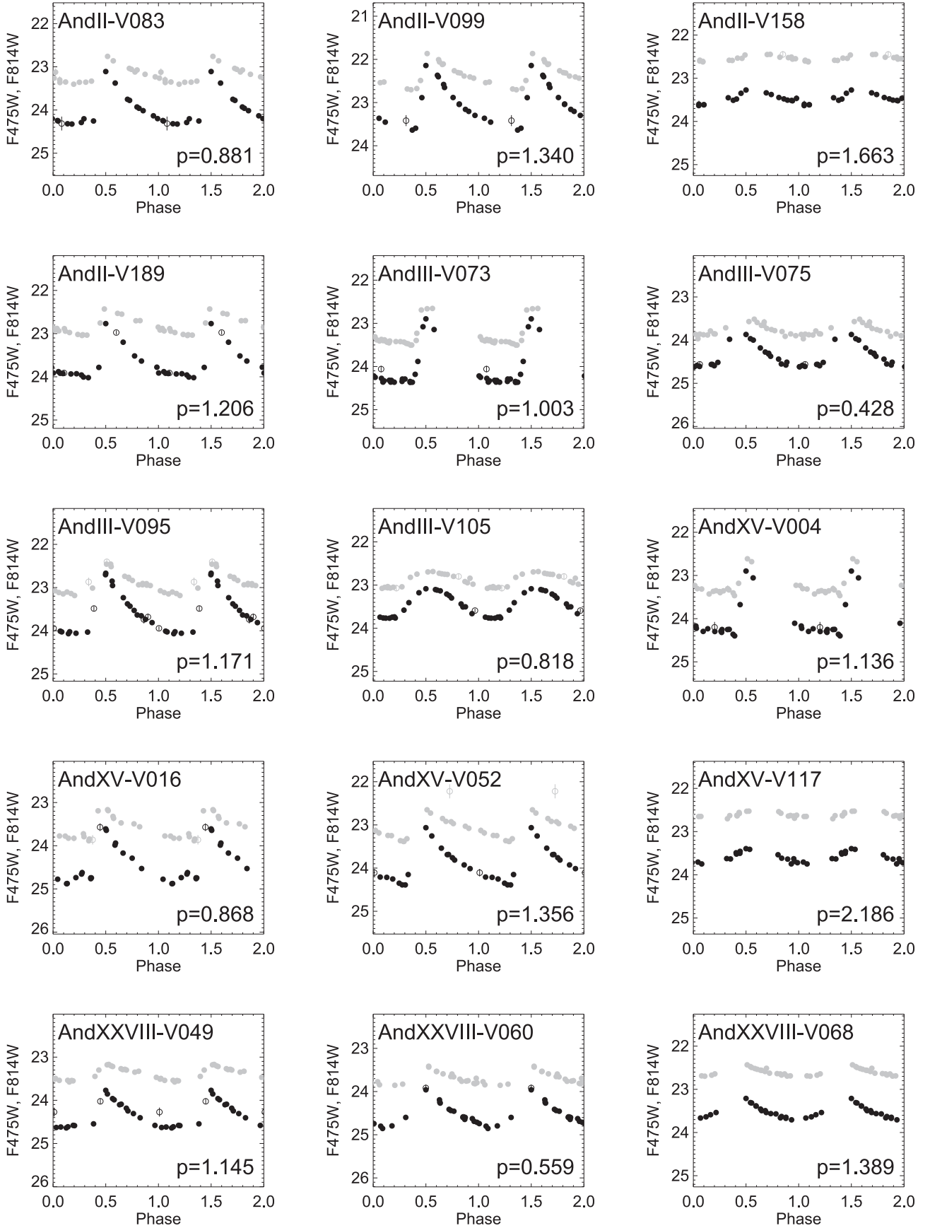
Figure 12. Light curves of member AC stars for four of the six ISLANDS galaxies in the F475W (black) and F814W (gray) bands. Periods (in days) are given in the lower right corner, while the name of the variable is displayed at the top of each panel. Open symbols show the data for which the uncertainties are larger than 3\sigma above the mean error of a given star; these data were not used in period and mean-magnitude calculations.
