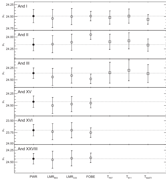
Figure 10. Summary of our derived distances. Circles report values based on RRL stars, while squares are based on the TRGB (provided only for the most massive galaxies, for which the TRGB could be reliably estimated). The filled circles and the dotted lines show the measurements based on the PWR, which are the final adopted distances. Open symbols show values obtained with the other methods for comparison.
