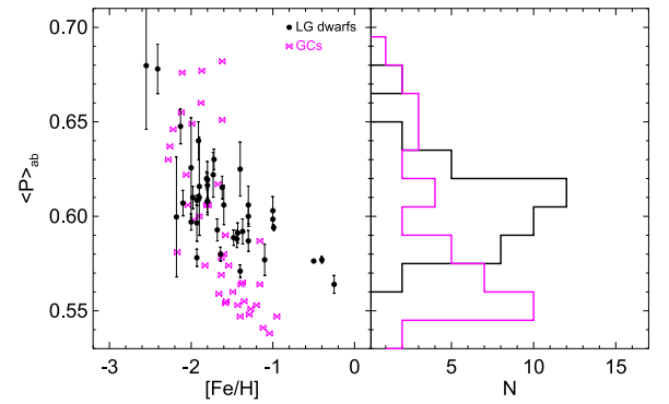
Figure 9. Left panel: \langle P_{ab} \rangle for a sample of 41 dwarf galaxies reported in Table 6 (black dots) as a function of [Fe/H] , compared to that of GCs (purple bowties). Right panel: period distribution of the sample of dwarf galaxies and GCs. The peak of the former occurs at a period typical of the Oo-intermediate system, while the latter peaks in the short-period regime, populated by Oo-I systems, which is devoid of galaxies.
