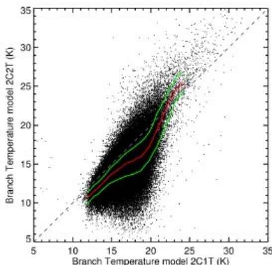
Figure 13. Relation between the average temperatures along the candidate branches estimated with the two approaches described in the text, i.e., the 2C1T and 2C2T modelling. The lines show the median (in red) and the quartiles (in green) of the 2C2T branch temperature distribution estimated in bins of 0.5 K.
