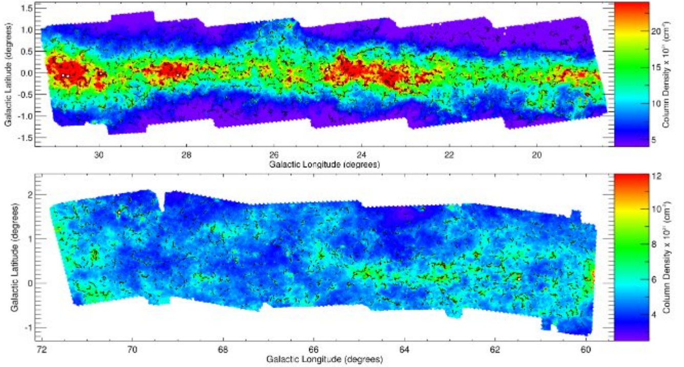
Figure 4. Example of candidate filaments identified in the two mosaics covering Galactic longitudes l = 19^\circ - 30^\circ and l = 60^\circ - 70^\circ shown in Figure 1. For sake of clarity, the figure shows only the branches as black lines.
