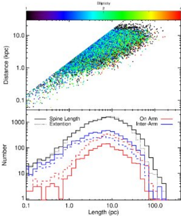
Figure 24. Top panel: Relation between the filament physical length and its assigned distance. The dashed line delimits the size corresponding to the cut-off criteria introduced in Sect. 4.1. Structures are shown with a colour code associated with their relative ellipticity e . Lower panel: Distributions of the physical sizes of the Hi-GAL filaments. The physical sizes are determined from two estimators (see Sect. 4.3): the length of the main axis, or angular length l^a , (continuous line) and the angular extension of the extended mask, l^e (dotted line). The red and blue lines show the l^a distributions for features associated to Galactic spiral arms and to inter-arm regions, respectively, for arm sizes of W = 600 pc (continuous lines) and W = 1 kpc (dashed lines).
