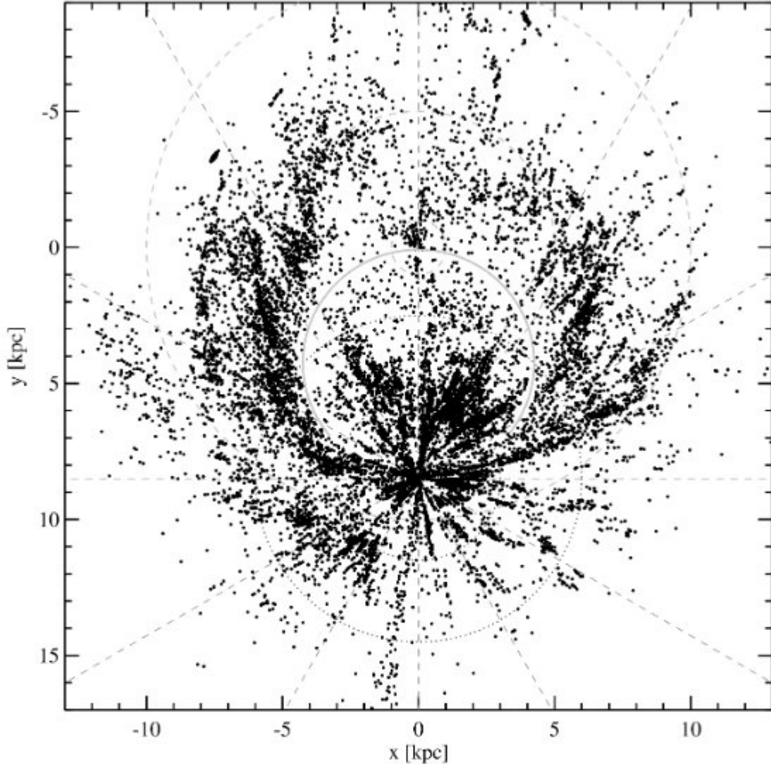
Figure 22. Top-down view of Milky Way with black dots indicating the location of 16,861 candidate filaments with a distance estimate. The dashed lines indicate line of sights separated by 30 degrees in longitude. The concentric circles refer to heliocentric distances equal to 1, 3, 6 kpc and to galactocentric distances of 1, 5, 10 kpc, with dotted and dashed lines respectively. The grey thick line identifies the position in the Galaxy where are located all the 1,528 filaments with RVs reported to their tangent point velocity, see text.
