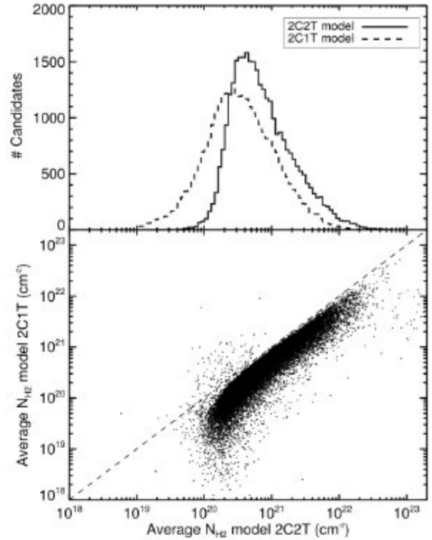
Figure 12. Top Panel: Distribution of the average column densities measured in the filament candidates with the two approaches described in the text, i.e., the 2C1T \bar{N}_{\text{H}_2}^{1\text{T}} (dashed line), and 2C2T \bar{N}_{\text{H}_2}^{2\text{T}} (solid line) modelling. Bottom Panel: Relation between the \bar{N}_{\text{H}_2}^{1\text{T}} and \bar{N}_{\text{H}_2}^{2\text{T}} .
