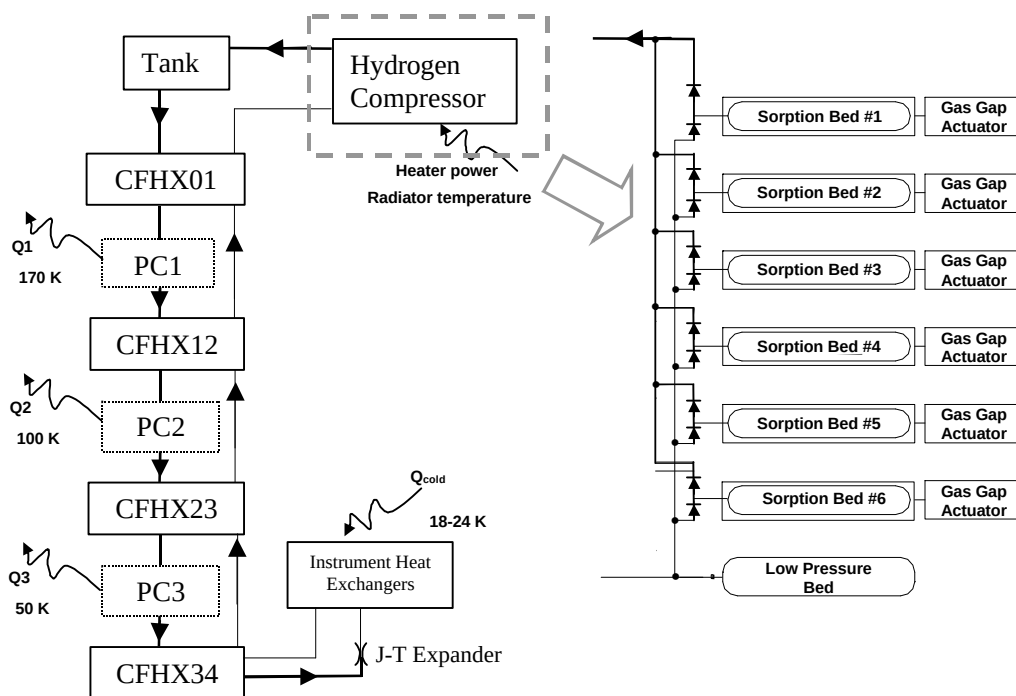
Figure 2-1. Planck Sorption Cooler Schematic
