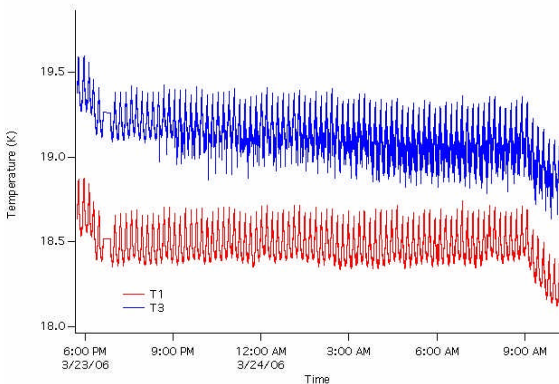
Figure 4-5 Reference Case LVHX's temperature value and stability
