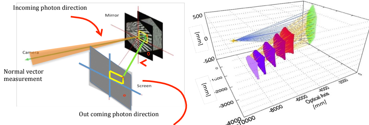
Figure 3 – Left: sketch of the measuring principle. Each point of the mirror can be associated with the position of a specific pixel on the screen. Knowing the distances between the screen, the camera and the mirror the normal vector to the surface at the considered point can be calculated. Right: Direct illumination of the mirror. A light source replaces the camera and the image reflected by the mirror is taken. The process is repeated for different screen positions. The dimensions and shapes of the reflected images are compared with the corresponding images obtained by means of the ray-tracing simulation of the reflection on a mirror with the measured slopes errors.
